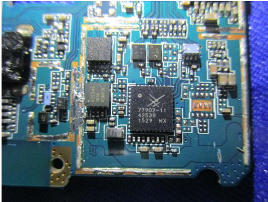
EUT –Wi-Fi&BT Chipset View
