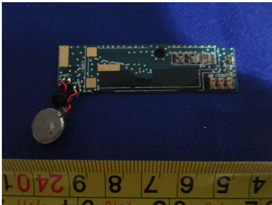
EUT –Voice PCB Top View
