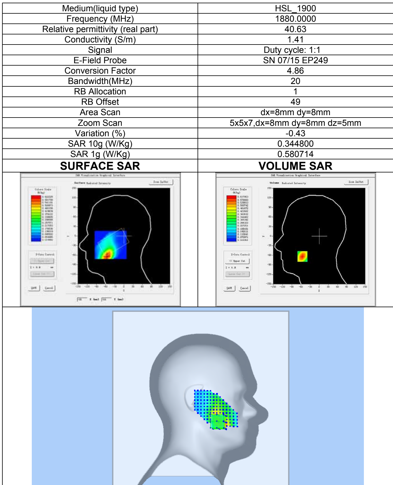
Plot 11:LTE BAND2, Middle channel (Left Head Cheek) Product Description:Mobile Phone Test Date: Jun. 08, 2017
