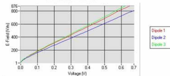
Calibration curves
