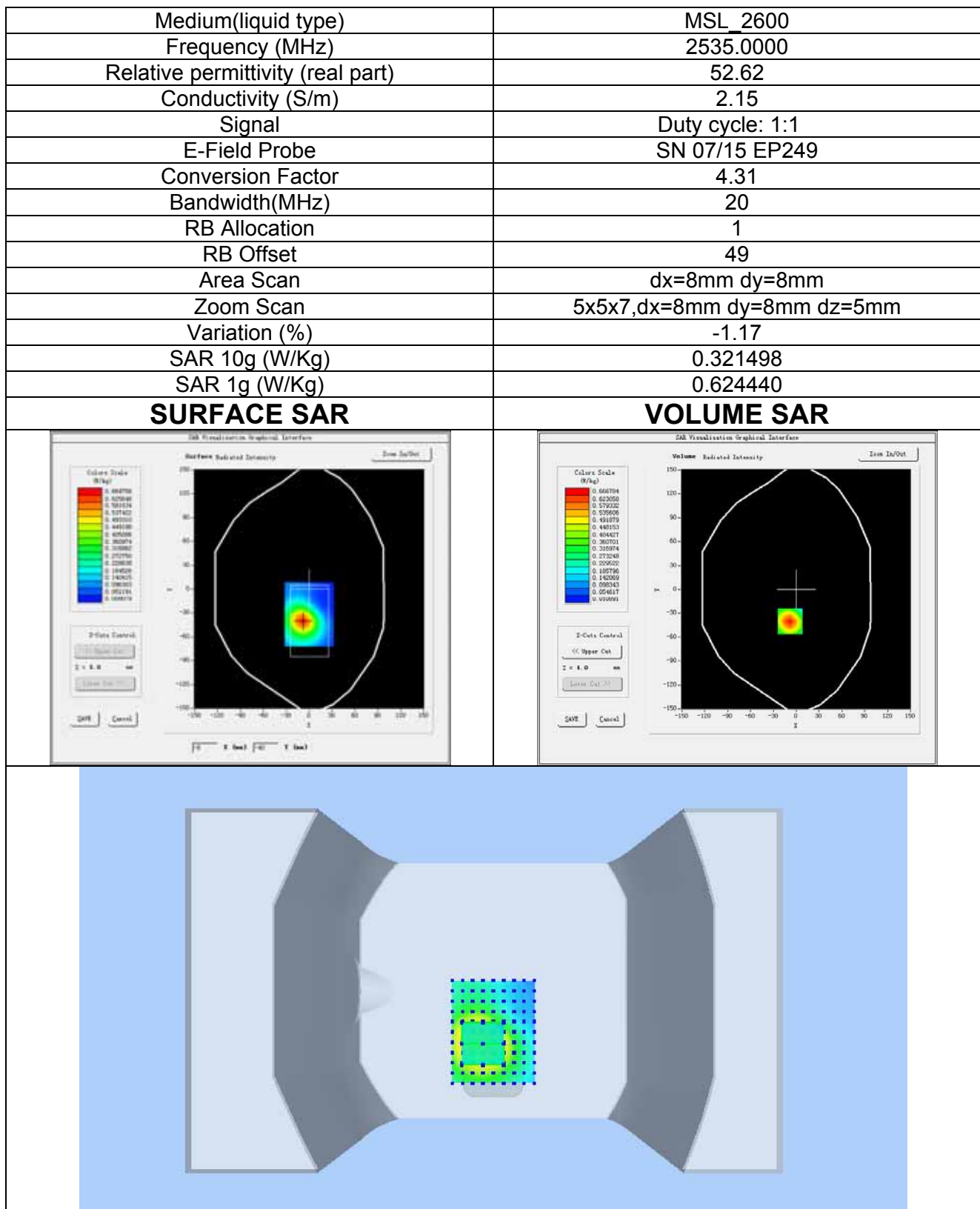
Plot 15:LTE BAND7, Middle channel (Body-worn, Back Surface) Product Description:Mobile Phone Test Date: Apr. 05, 2017
