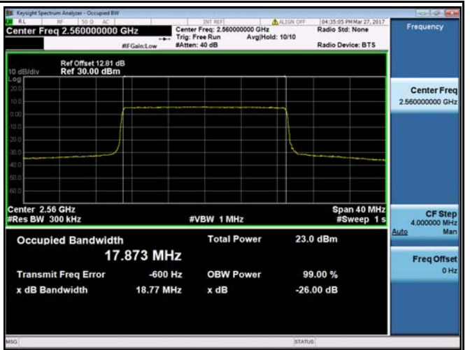
LTE band 7 - High CH 16QAM-20
