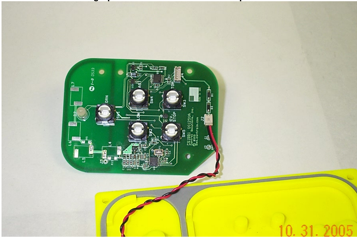
Photograph of Transmitter Board – Component Side
