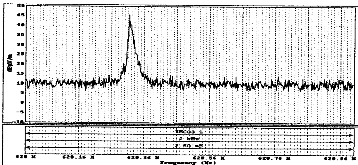
Fig.7. Emission from unit 1 at its second harmonic. The maximum emission was found to be vertically polarized and at 1.0-m height.
