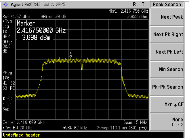
Low Ch-2418MHz_10MHz BW Spectral Density_Port 2
