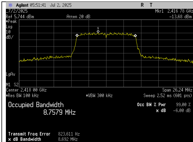
Low Ch_2418MHz_10MHz BW_Occupied Bandwidth_-6dB_Port 1
