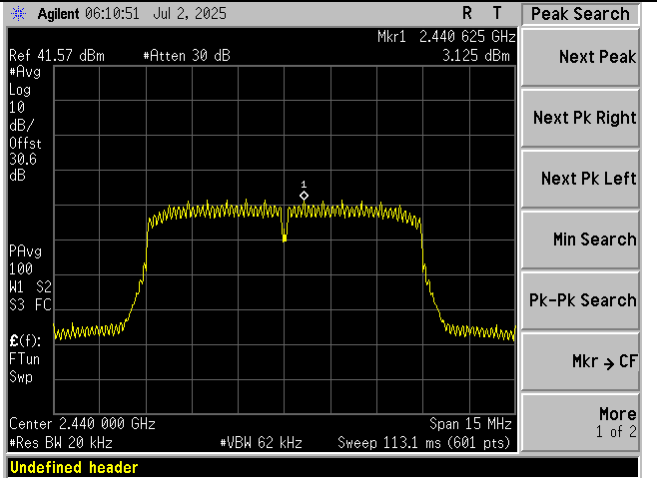
Mid Ch-2440MHz_10MHz BW Spectral Density_Port 2
