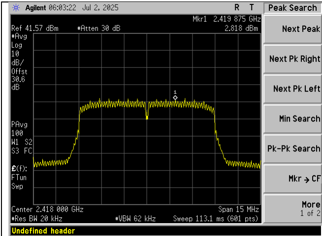
Low Ch-2418MHz_10MHz BW Spectral Density_Port 1
