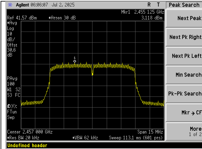
High Ch-2457MHz_10MHz BW Spectral Density_Port 1
