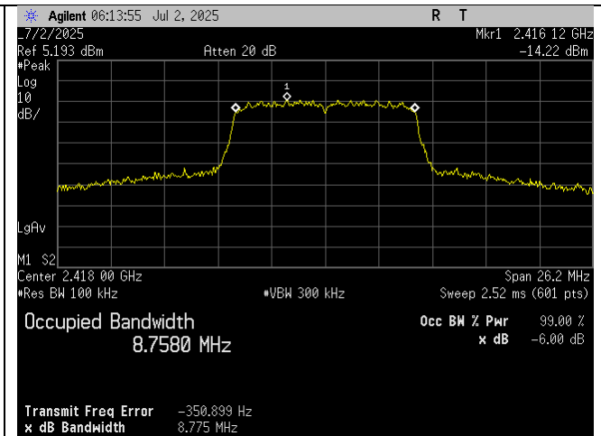
Low Ch_2418MHz_10MHz BW_Occupied Bandwidth_-6dB_Port 2
