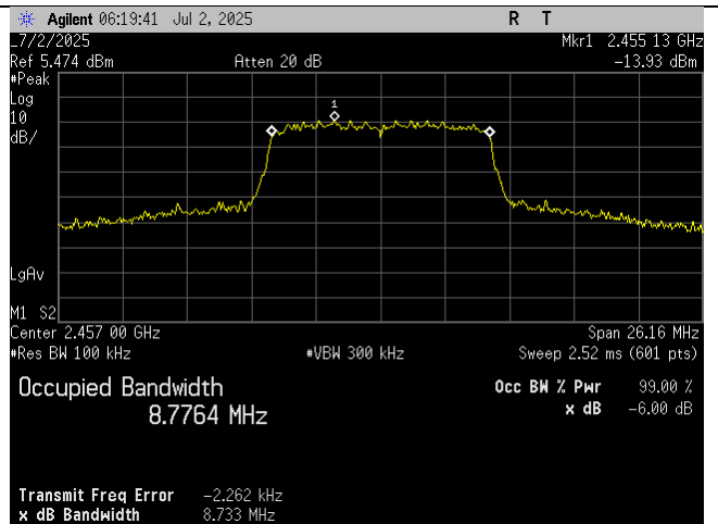
High Ch_2457MHz_10MHz BW_Occupied Bandwidth_-6dB_Port 2
