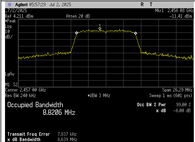
High Ch_2457MHz_10MHz BW_Occupied Bandwidth_99 percent_Port 1
