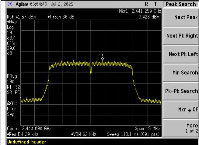
Mid Ch-2440MHz_10MHz BW Spectral Density_Port 1
