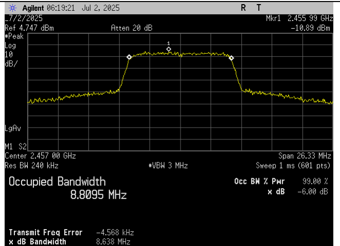
High Ch_2457MHz_10MHz BW_Occupied Bandwidth_99 percent_Port 2
