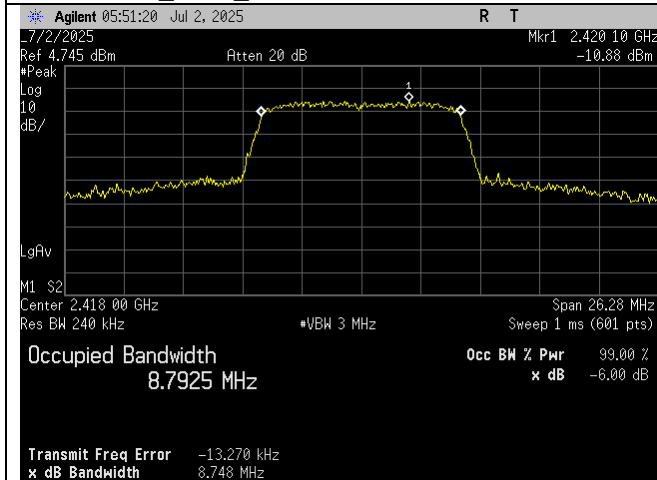
Low Ch_2418MHz_10MHz BW_Occupied Bandwidth_99 percent_Port 1
