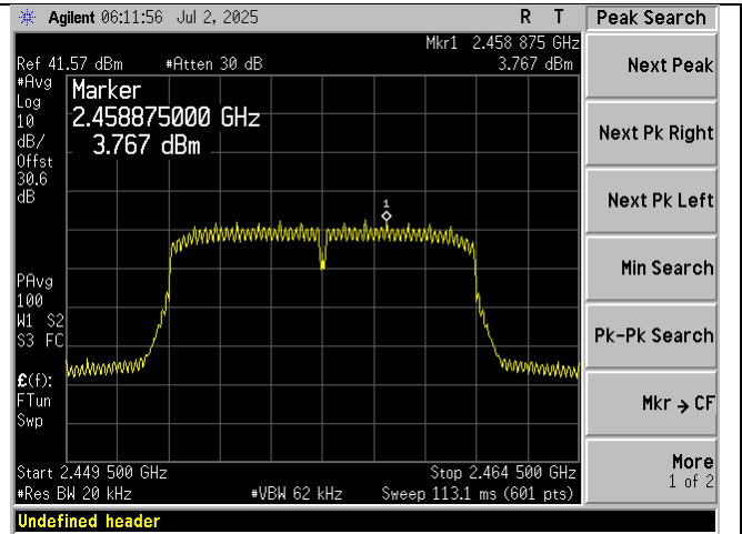
High Ch-2457MHz_10MHz BW Spectral Density_Port 2
