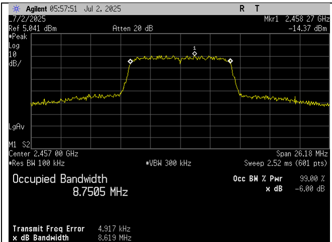
High Ch_2457MHz_10MHz BW_Occupied Bandwidth_-6dB_Port 1
