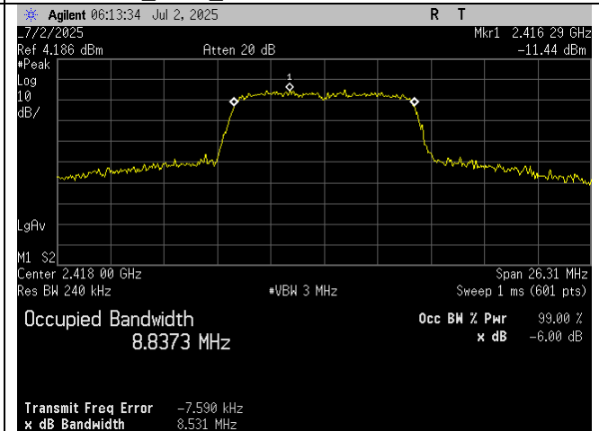
Low Ch_2418MHz_10MHz BW_Occupied Bandwidth_99 percent_Port 2
