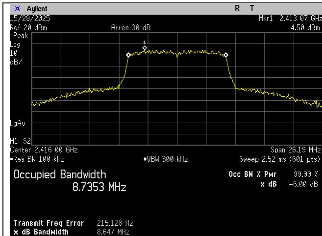
Low Ch_2416MHz_10MHz BW_Occupied Bandwidth_-6dB_Port 1
