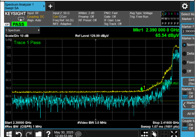
Low Ch 2416 MHz Lower Band Edge Peak Vertical
