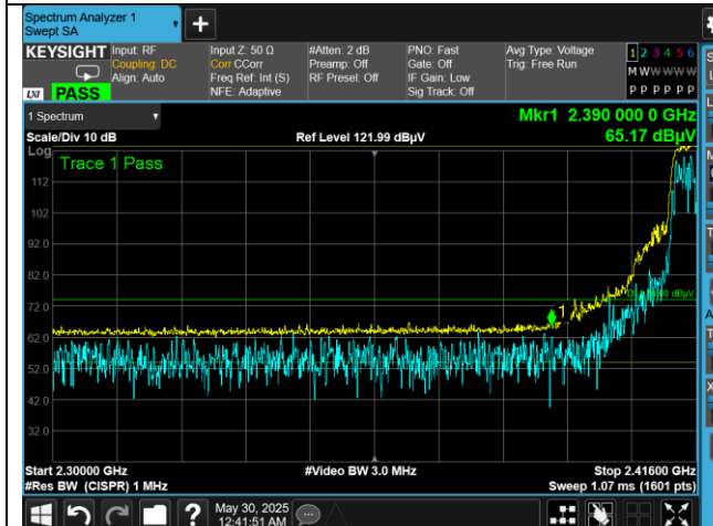
Low Ch 2416 MHz Lower Band Edge Peak Horizontal
