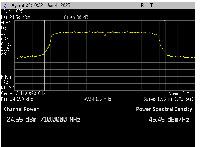
Mid Ch_2440MHz_10MHz BW_Output Power_Port 2
