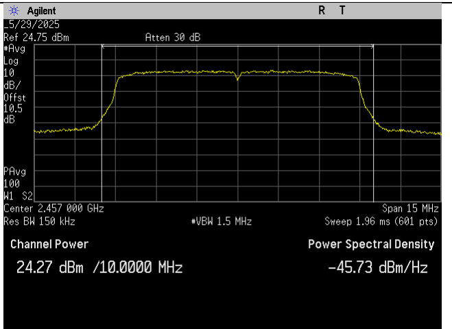
High Ch_2457MHz_10MHz BW_Output Power_Port 2
