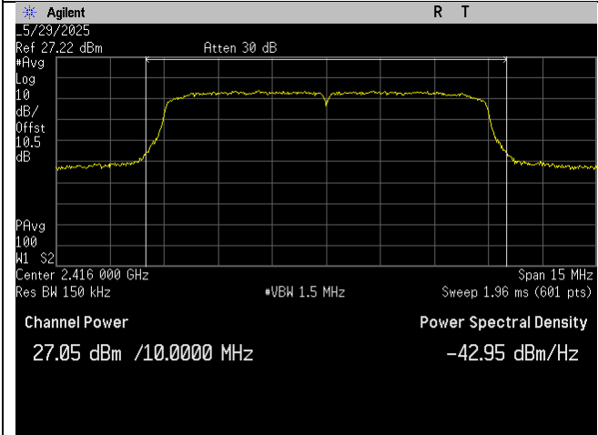
Low Ch_2416MHz_10MHz BW_Output Power_Port 1
