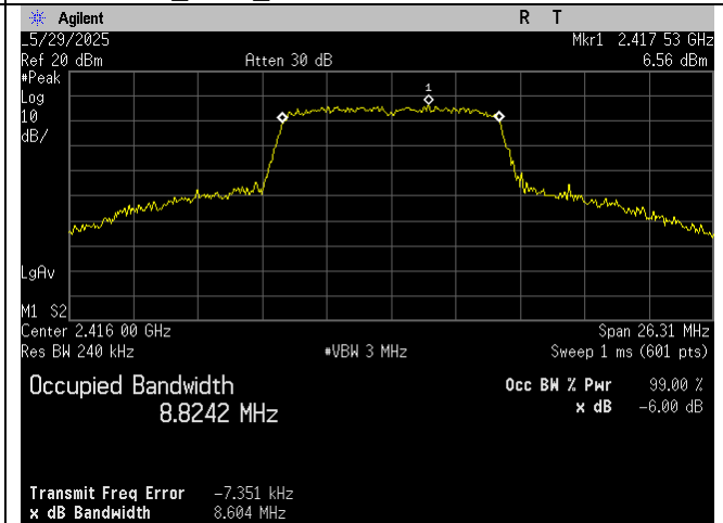
Low Ch_2416MHz_10MHz BW_Occupied Bandwidth_99 percent_Port 2
