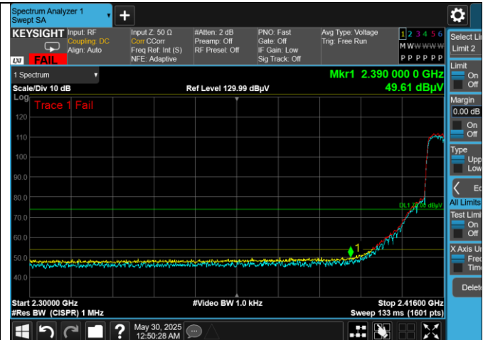
Low Ch 2416 MHz Lower Band Edge Average Vertical
