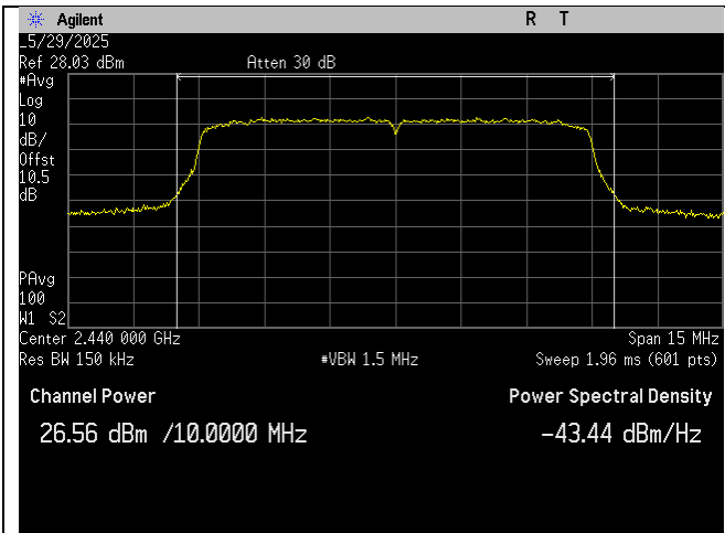
Mid Ch_2440MHz_10MHz BW_Output Power_Port 1
