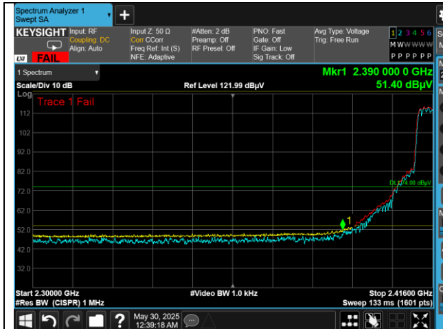
Low Ch 2416 MHz Lower Band Edge Average Horizontal
