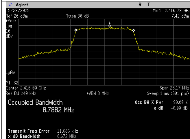
Low Ch_2416MHz_10MHz BW_Occupied Bandwidth_99 percent_Port 1
