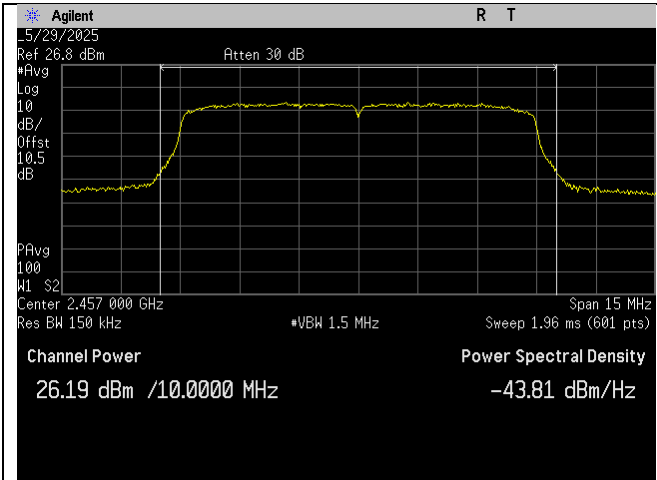
High Ch_2457MHz_10MHz BW_Output Power_Port 1
