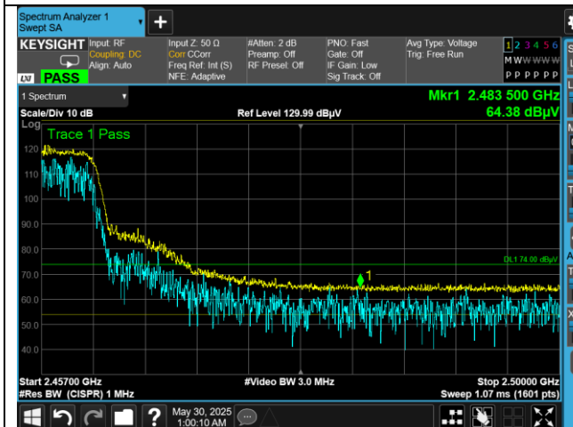
High Ch 2457 MHz Upper Band Edge Peak Horizontal
