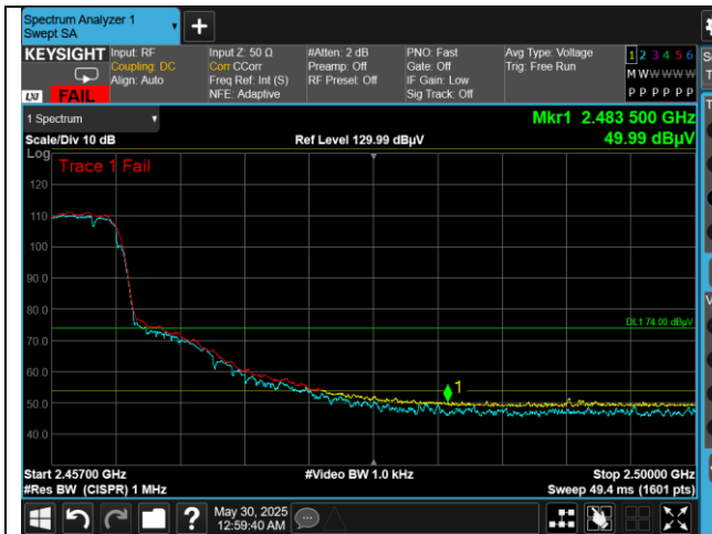
High Ch 2457 MHz Upper Band Edge Average Horizontal
