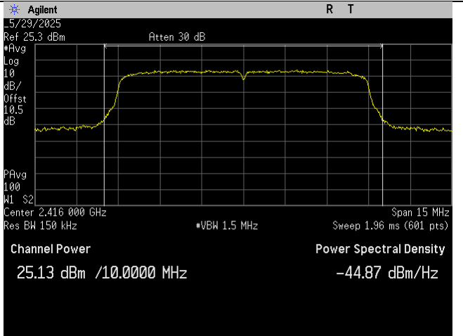
Low Ch_2416MHz_10MHz BW_Output Power_Port 2
