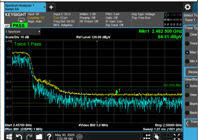
High Ch 2457 MHz Upper Band Edge Peak Vertical
