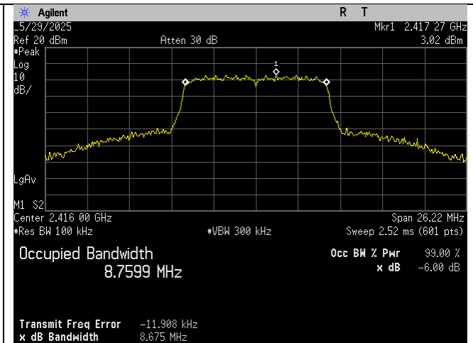
Low Ch_2416MHz_10MHz BW_Occupied Bandwidth_-6dB_Port 2
