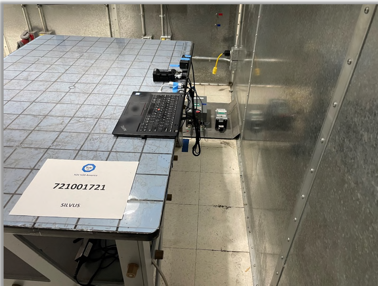
Conducted Emissions Back View Test Setup
