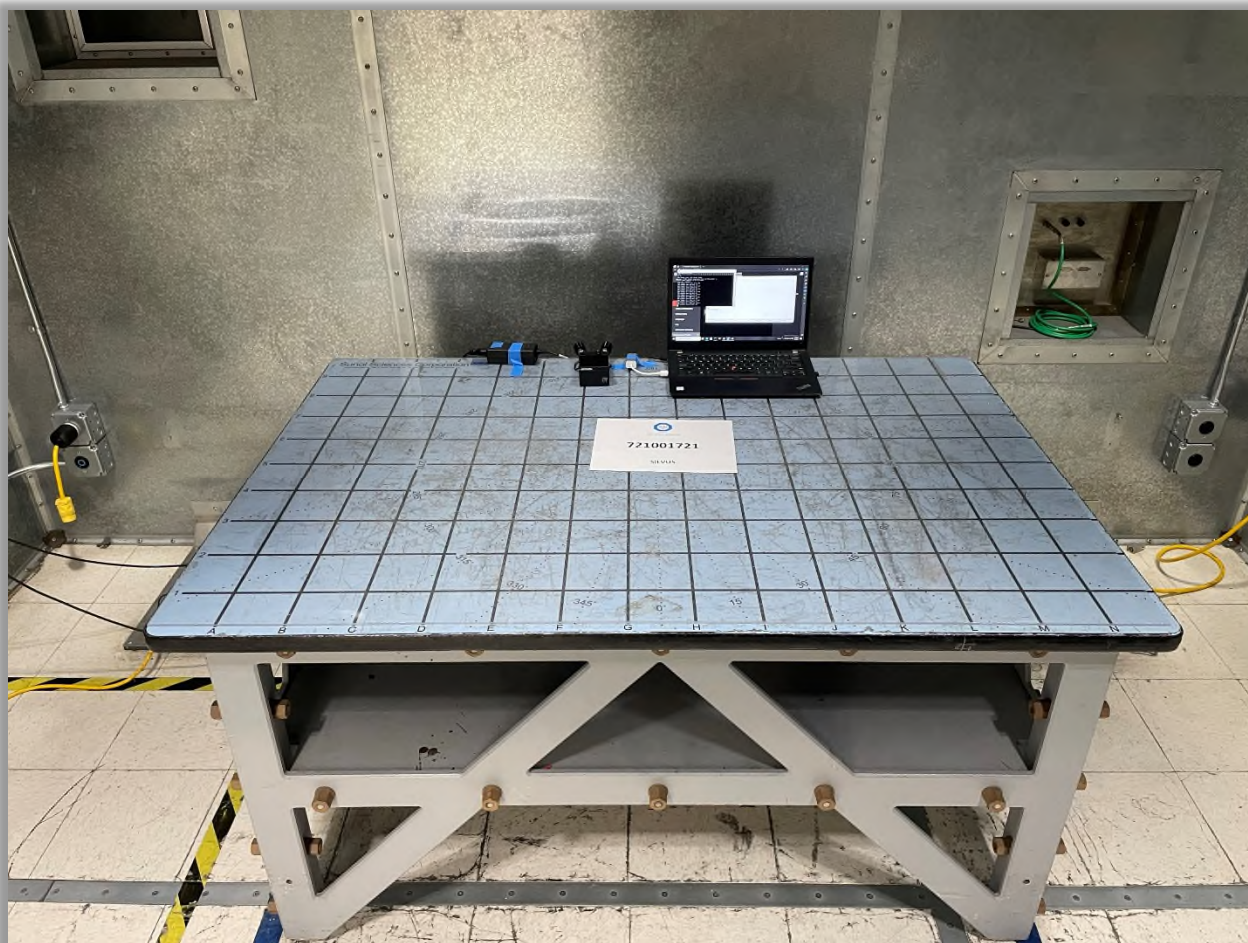
Conducted Emissions Back Front Test Setup
