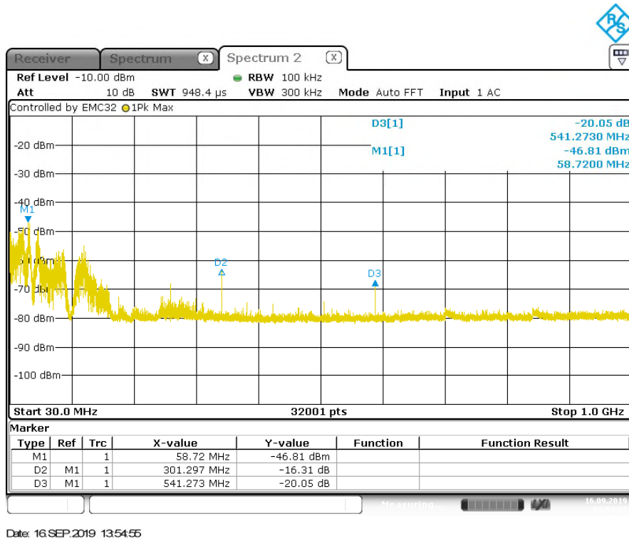
Note: Emissions above the noise floor are from the digital sections of the DUT and not associated with the radio. Figure A-1: 30MHz-1GHz
