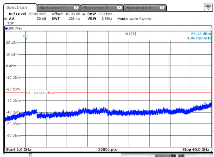
Figure 7.6.2-4: MCH – 1GHz–40GHz
