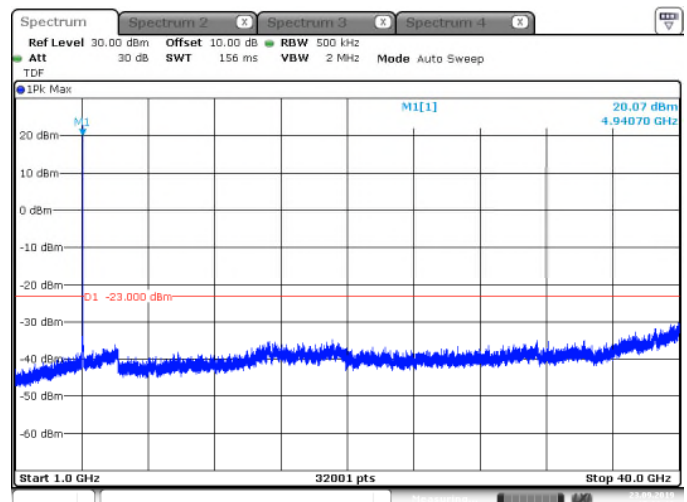
Figure 7.6.2-2: LCH – 1GHz–40GHz
