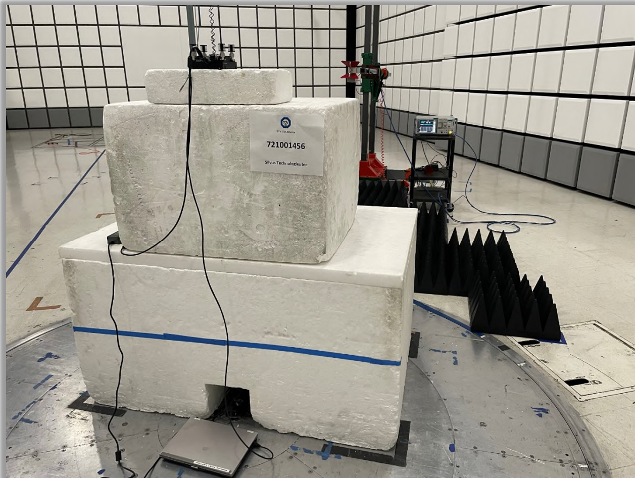
Radiated Emissions Test Setup (1GHz to 18GHz)
