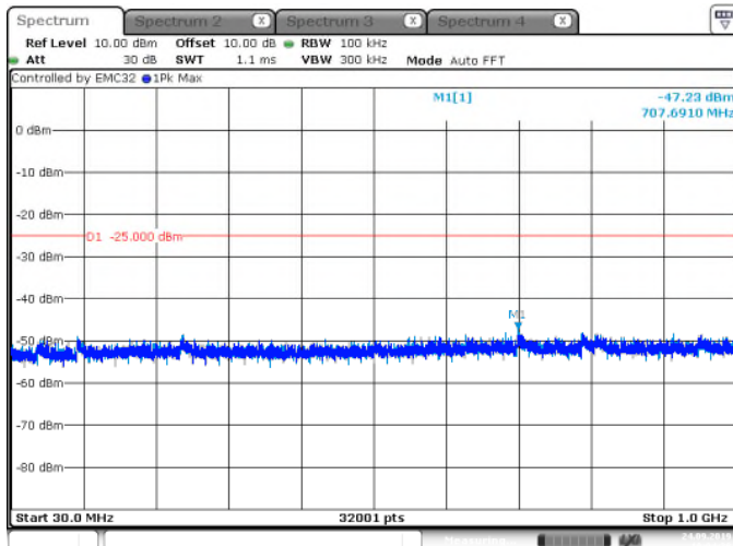
Figure 7.6.2-3: MCH – 30MHz–1GHz
