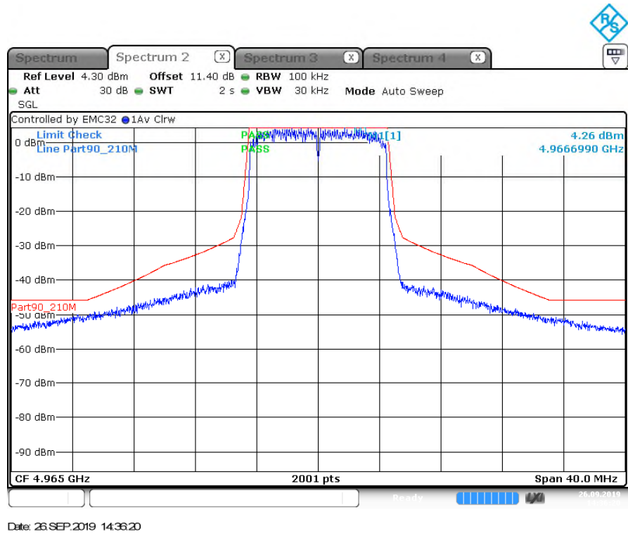
Figure 7.1.2-3: Mask M – Middle Channel
