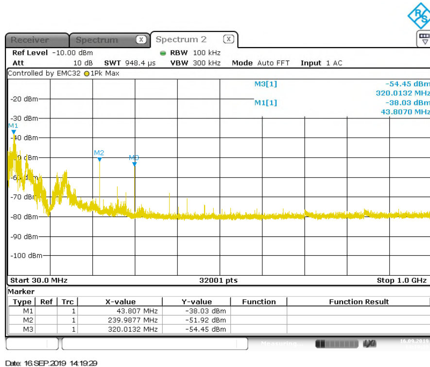
Figure A-1: 30MHz-1GHz
