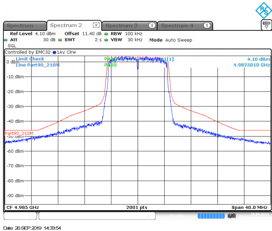
Figure 7.1.2-4: Mask M – High Channel
