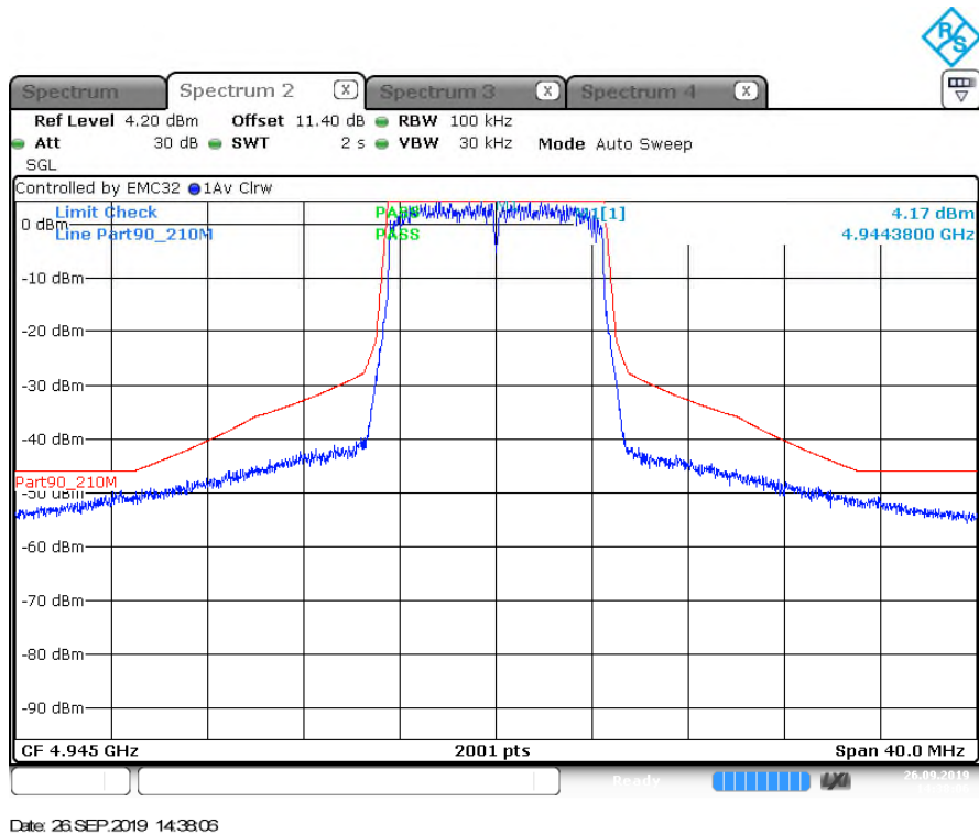
Figure 7.1.2-2: Mask M – Low Channel
