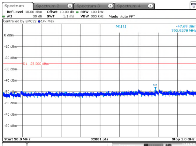
Figure 7.6.2-1: LCH – 30MHz–1GHz
