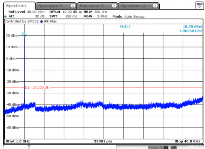
Figure 7.6.2-4: MCH – 1GHz–40GHz
