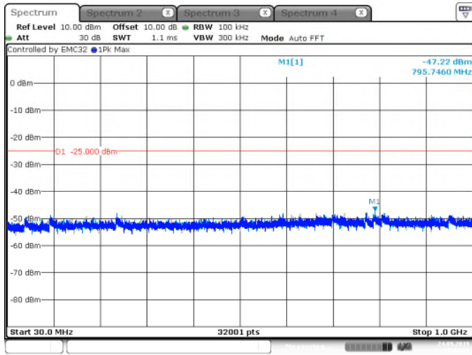
Figure 7.6.2-5: HCH - 30MHz-1GHz
