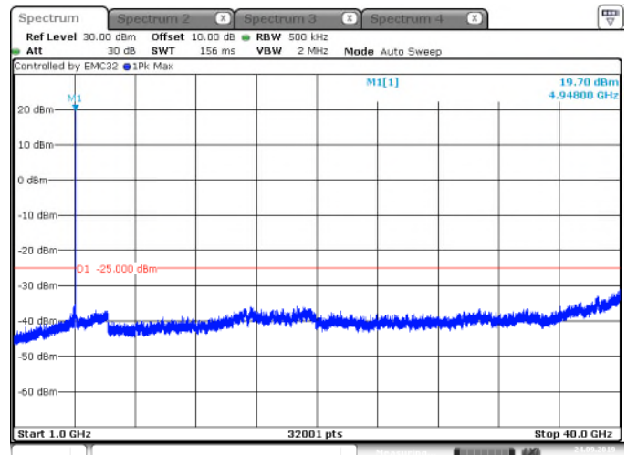
Figure 7.6.2-2: LCH – 1GHz–40GHz
