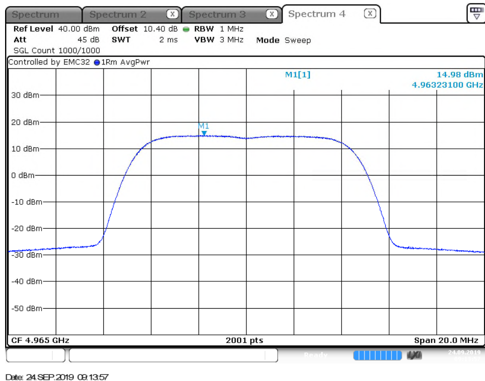
Figure 7.3.2-1: Sample PSD Plot
