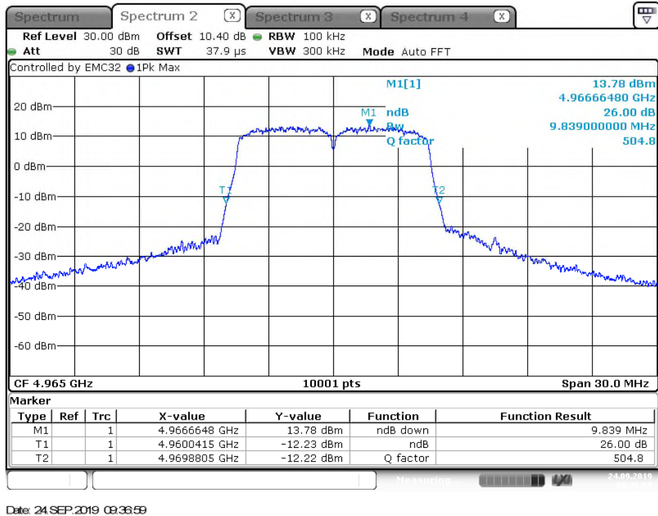
Figure 7.1.2-1: Sample Plot - 26dB BW
