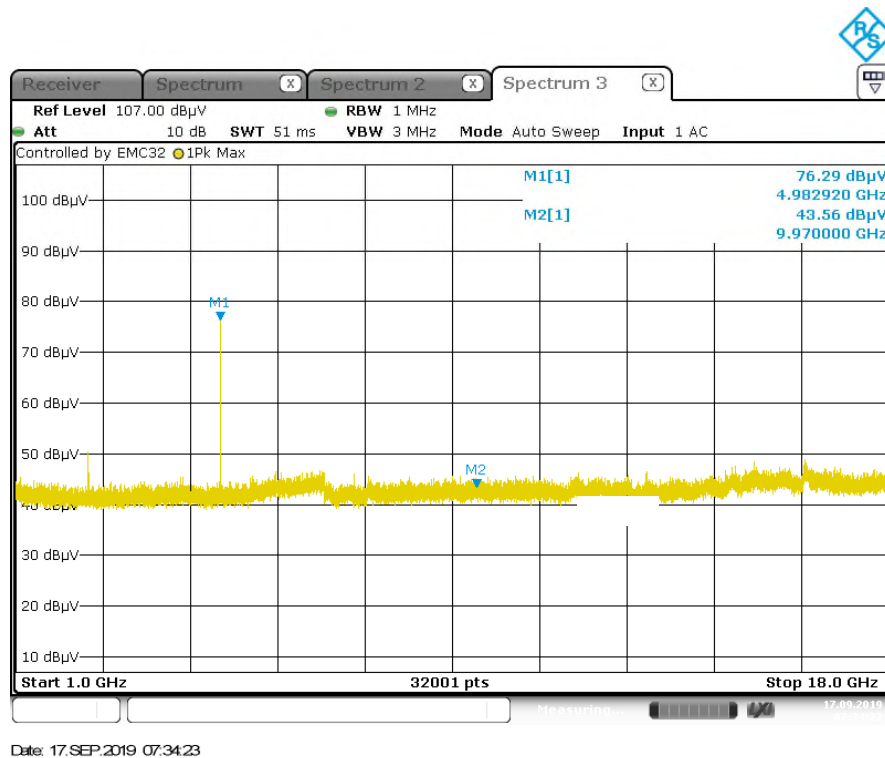
Figure A-2: 1GHz-18GHz
