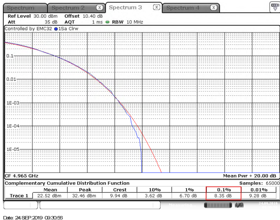
Figure 7.4.2-1: PAPR Plot
