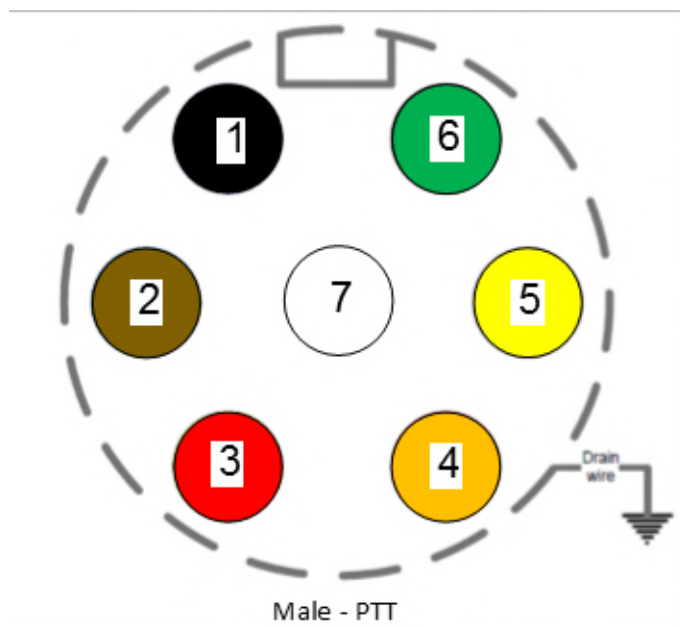
Figure 10 SC4400E PTT Pinout Diagram (Cable Side)
