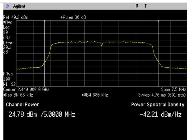
2440MHz_5MHz BW_Output Power_Port 2
