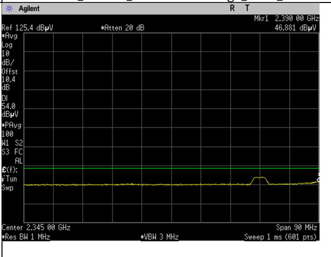
2412MHz_15.209_Lower Band Edge_Avg_Port 2
