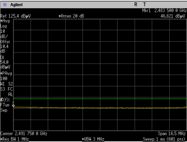
2462MHz_15.209_Upper Band Edge_Avg_Port 2
