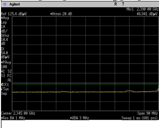
2412MHz_15.209_Lower Band Edge_Avg_Port 1
