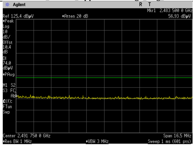
2462MHz_15.209_Upper Band Edge_Avg_Port 1
