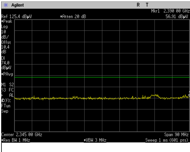
2412MHz_15.209_Lower Band Edge_Peak_Port 2
