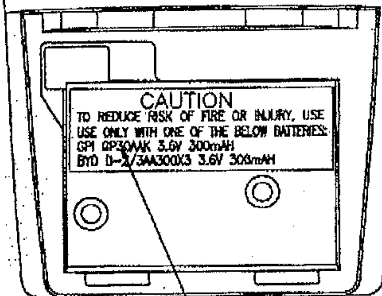
LABEL-BATTERY
