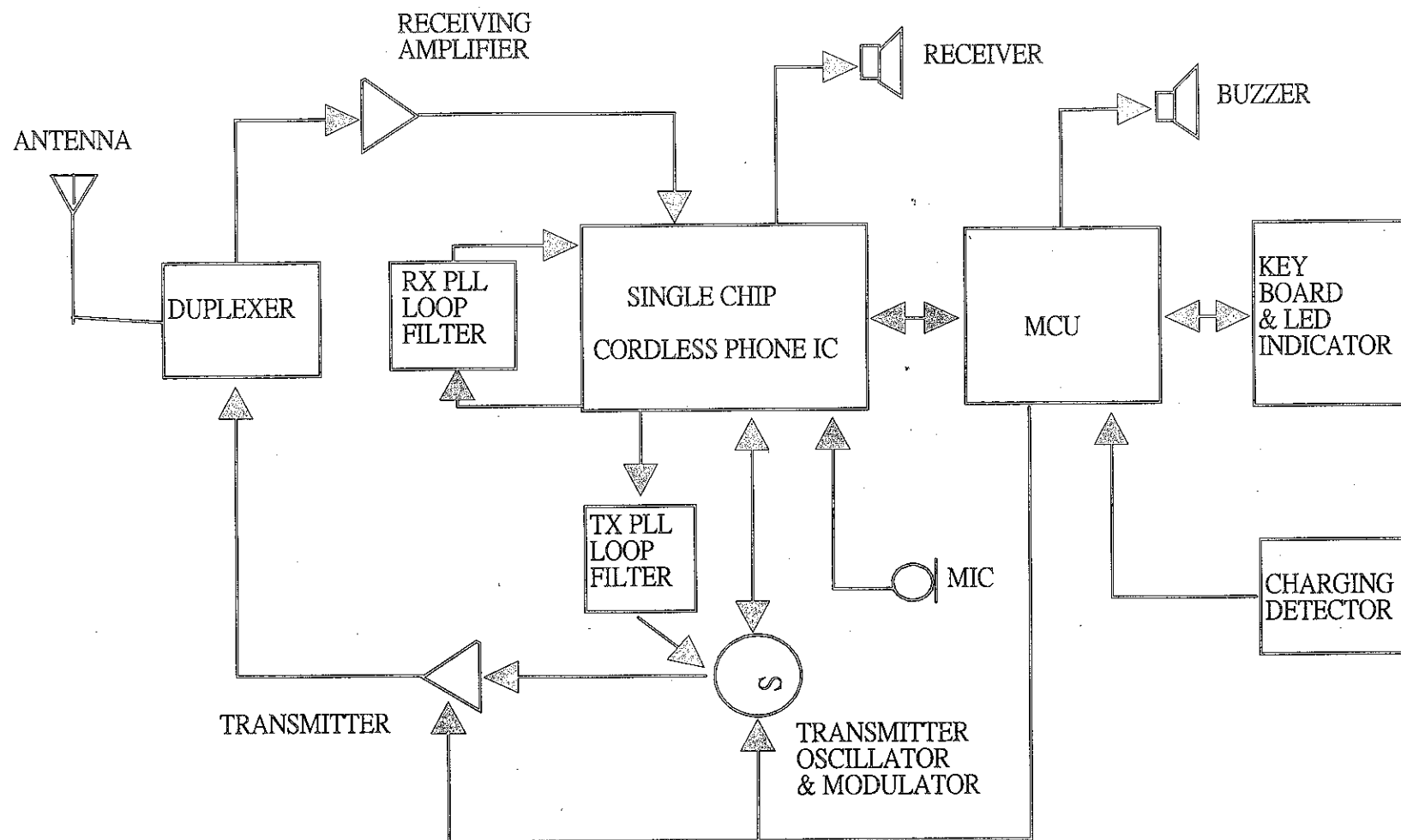
BEF25 HEADSET BLOCK DIAGRAM
