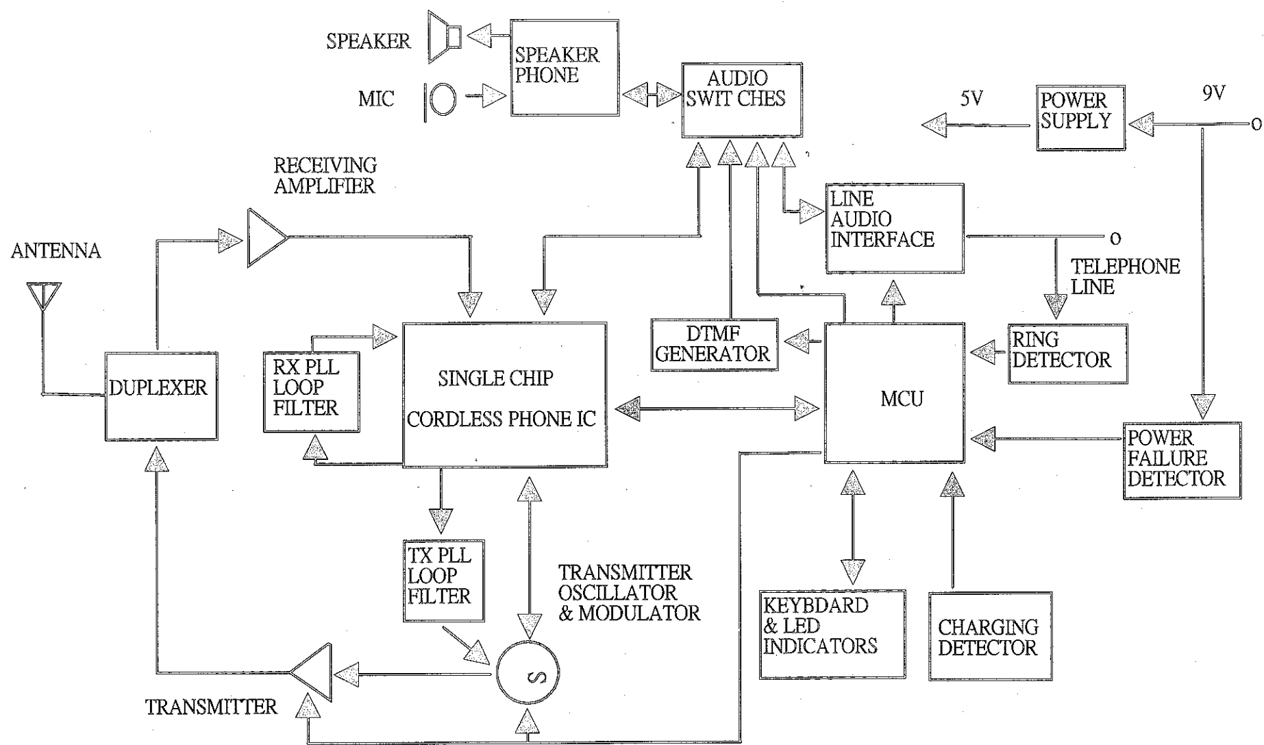
BEF25 BASE UNIT BLOCK DIAGRAM
