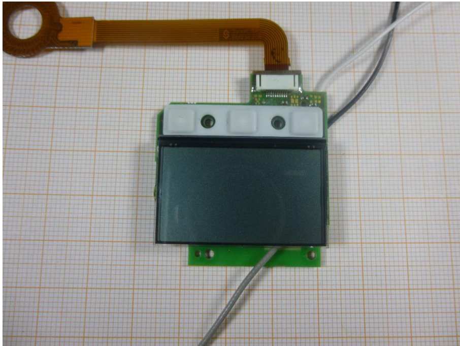
Photo 4: PCB front side view with display
