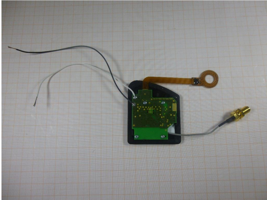
Photo 1: PCB back side view
