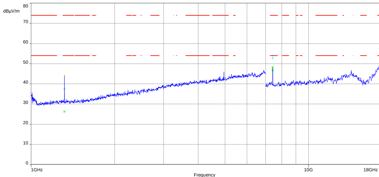
Plot 5: 1 GHz to 18 GHz, TX mode, 2475 MHz, vertical & horizontal polarization
