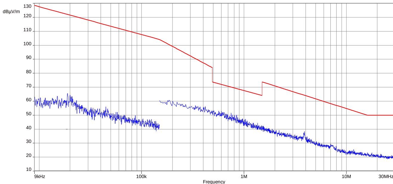
Plot 1: 9 kHz to 30 MHz, 2403 MHz, transmit mode
