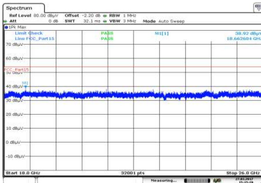
Plot 2: 18 GHz to 26 GHz, TX mode, 2403 MHz, vertical & horizontal polarization
