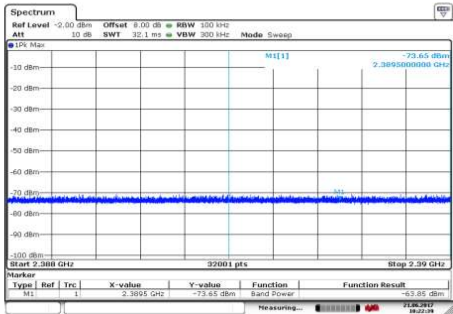
Plot 1: Lower band edge
