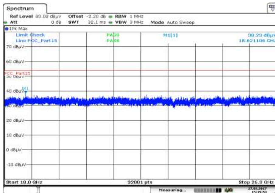
Plot 4: 18 GHz to 26 GHz, TX mode, 2439 MHz, vertical & horizontal polarization
