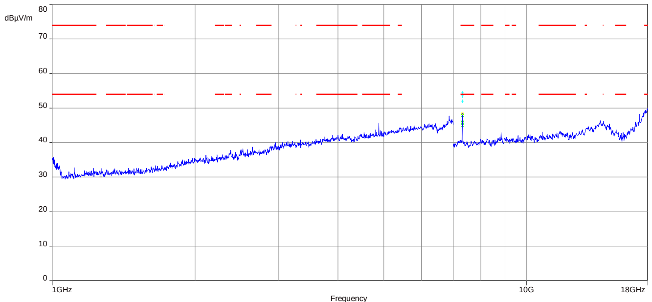
Plot 3: 1 GHz to 18 GHz, TX mode, 2439 MHz, vertical & horizontal polarization
