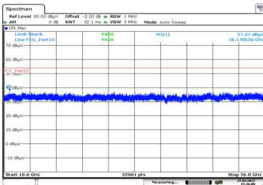
Plot 6: 18 GHz to 26 GHz, TX mode, 2475 MHz, vertical & horizontal polarization
