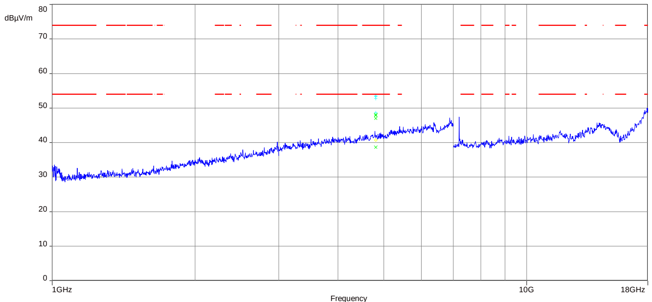
Plot 1: 1 GHz to 18 GHz, TX mode, 2403 MHz, vertical & horizontal polarization
