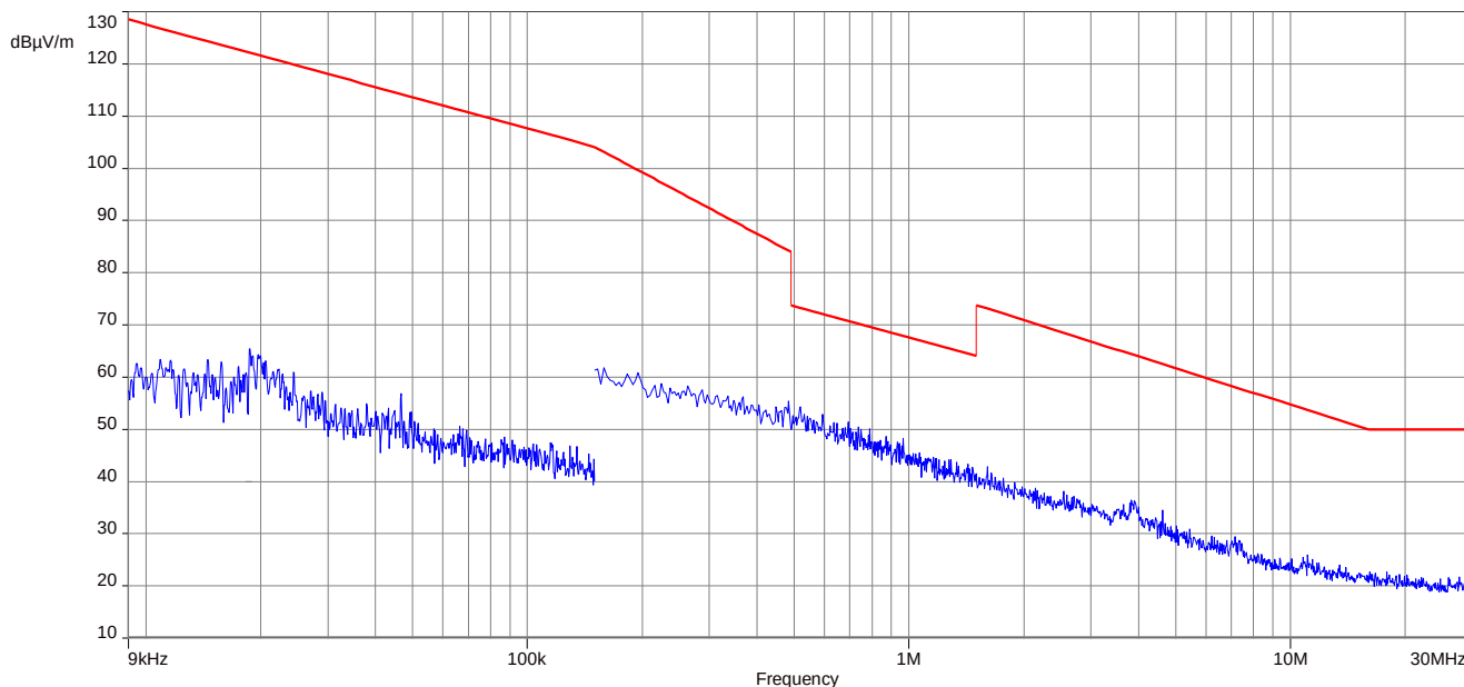
Plot 2: 9 kHz to 30 MHz, 2439 MHz, transmit mode
