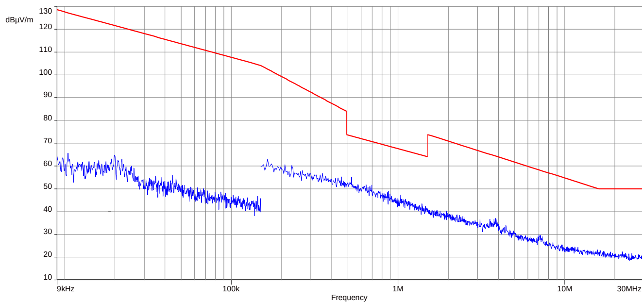
Plot 3: 9 kHz to 30 MHz, 2475 MHz, transmit mode
