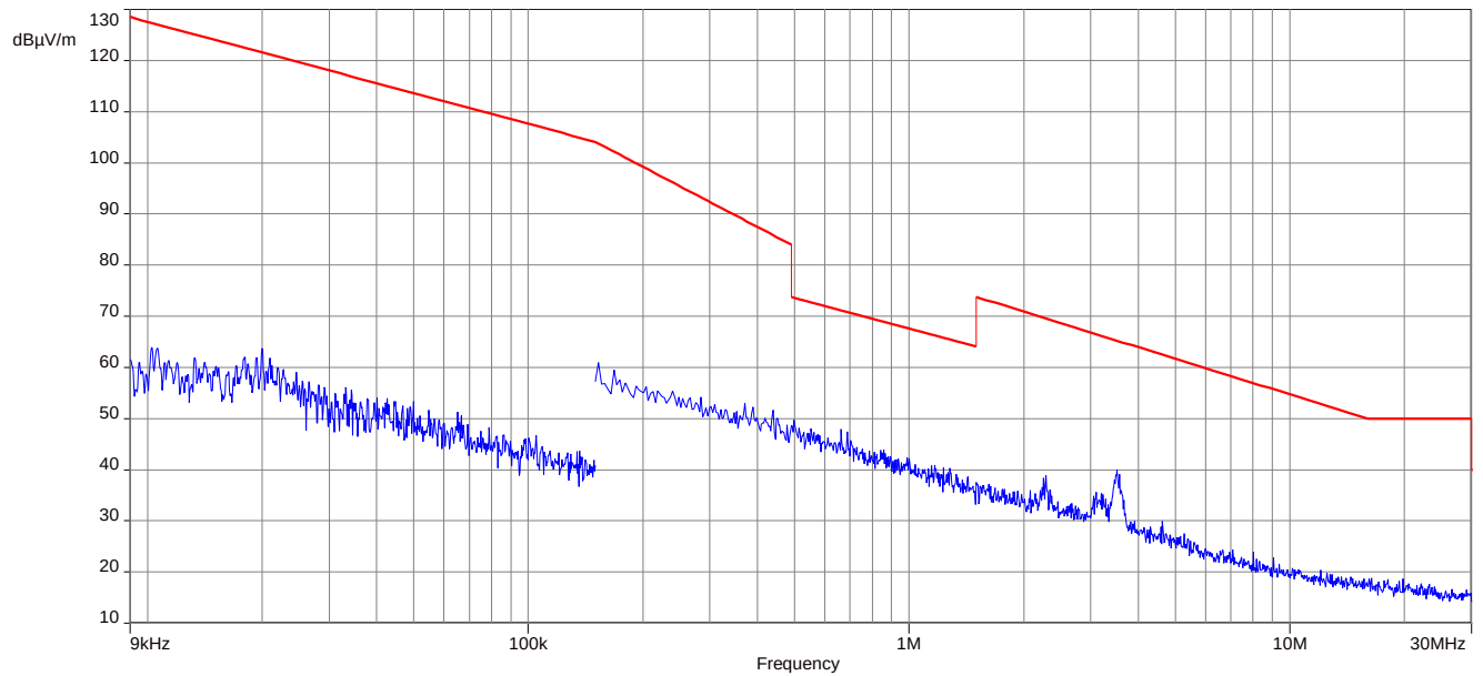
Plot 1: 9 kHz to 30 MHz, low channel
