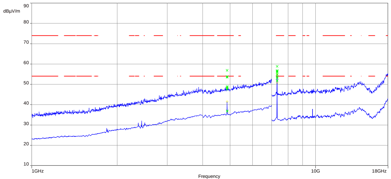
Plot 3: 1 GHz to 18 GHz, mid channel, vertical & horizontal polarization
