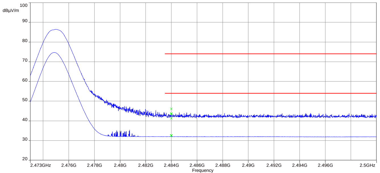
Plot 2: Upper restricted band
