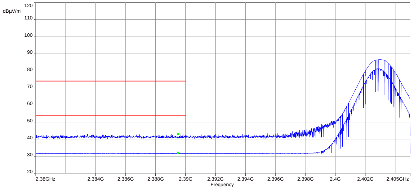
Plot 1: Lower restricted band
