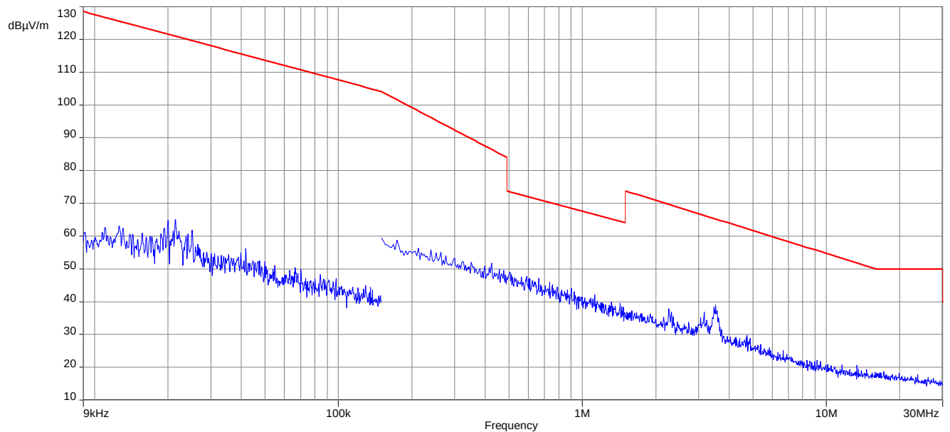
Plot 2: 9 kHz to 30 MHz, mid channel
