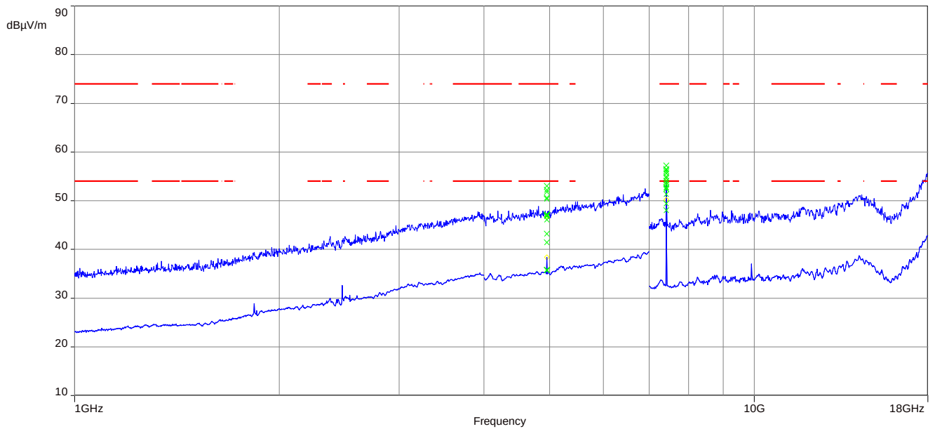
Plot 5: 1 GHz to 18 GHz, high channel, vertical & horizontal polarization
