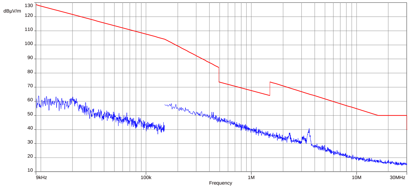
Plot 3: 9 kHz to 30 MHz, high channel
