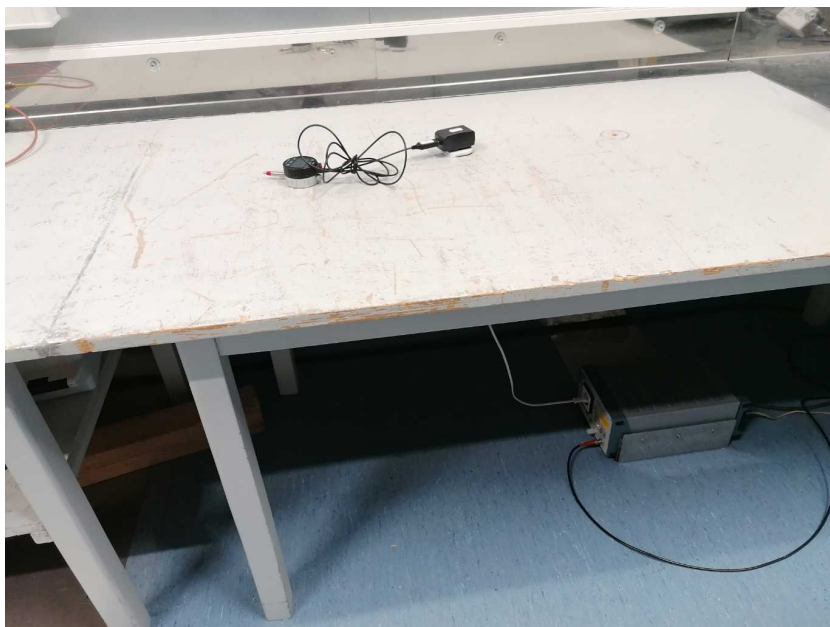
Photo 12: AC conducted emission test setup
