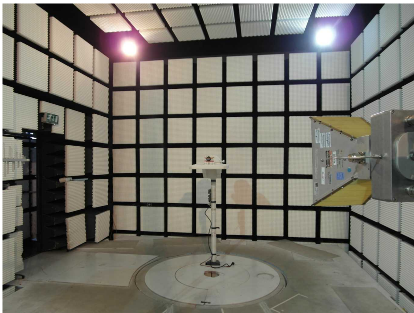
Photo 8: EUT at the anechoic chamber
