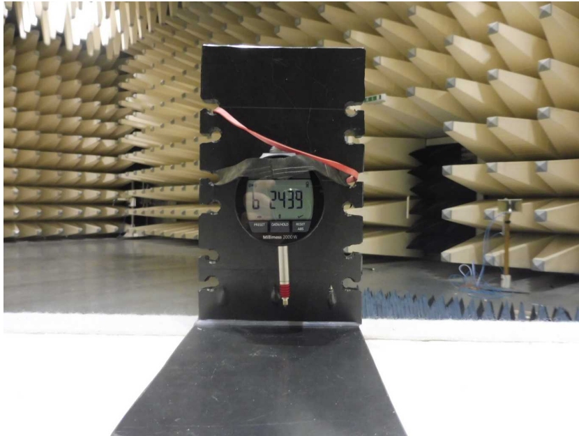
Photo 11: EUT at the semi-anechoic chamber
