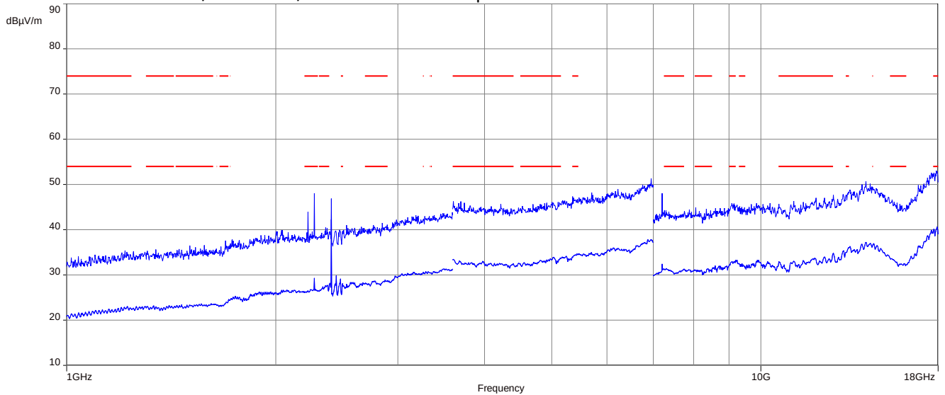
Plot 1: 1 GHz to 18 GHz, 2403 MHz, vertical & horizontal polarization
