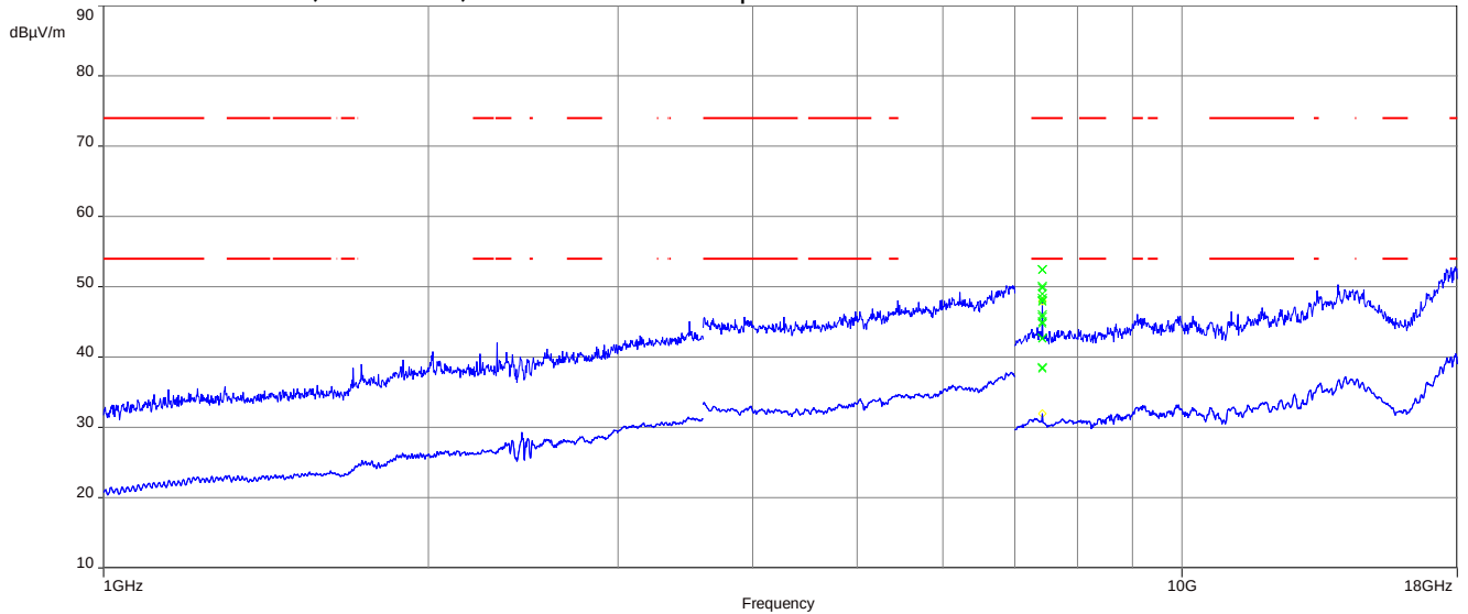
Plot 3: 1 GHz to 18 GHz, 2475 MHz, vertical & horizontal polarization
