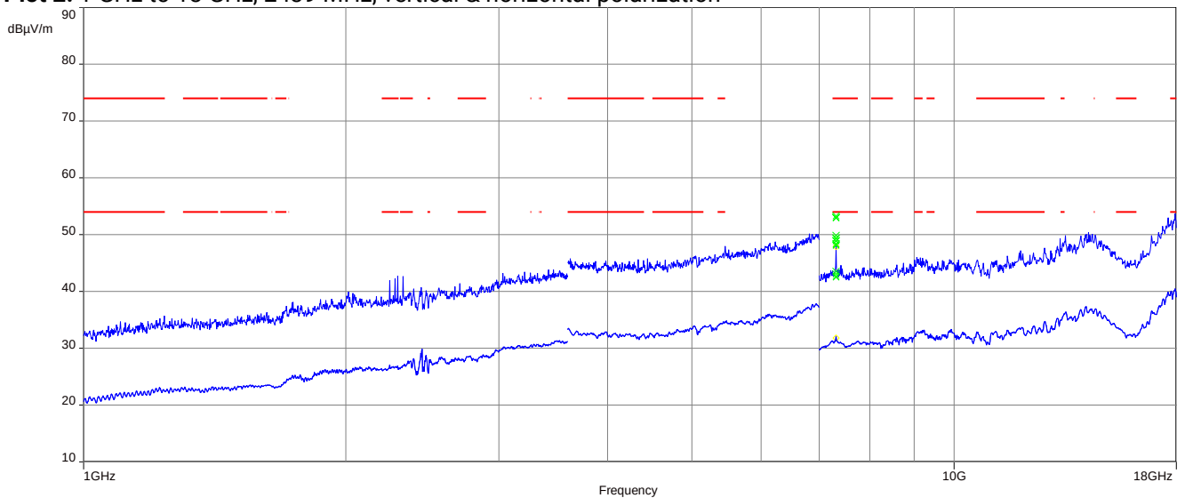
Plot 2: 1 GHz to 18 GHz, 2439 MHz, vertical & horizontal polarization
