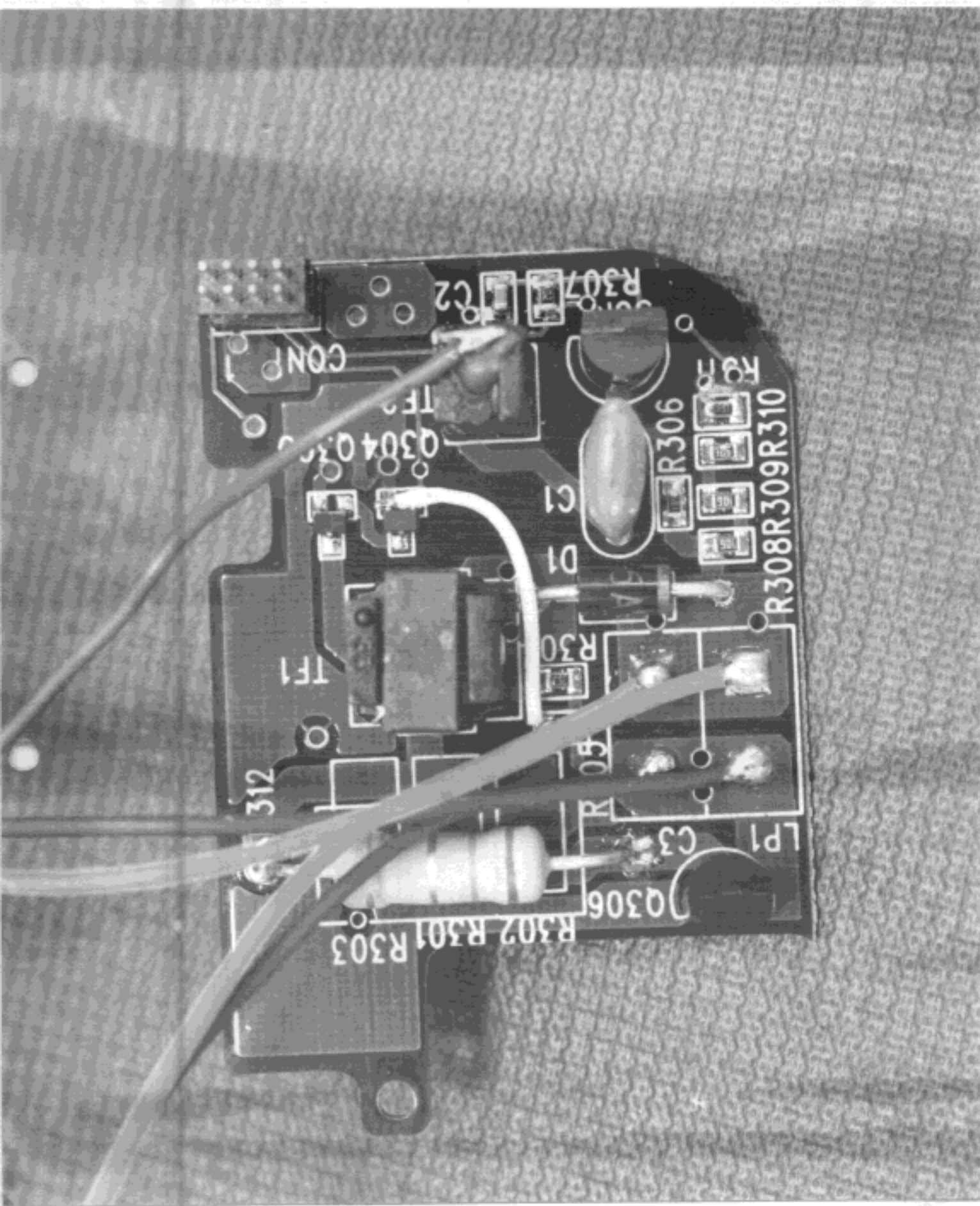
FCC ID: N3DLARGAND601A PHOTO 10. EUT COMPONENT SIDE VIEW
