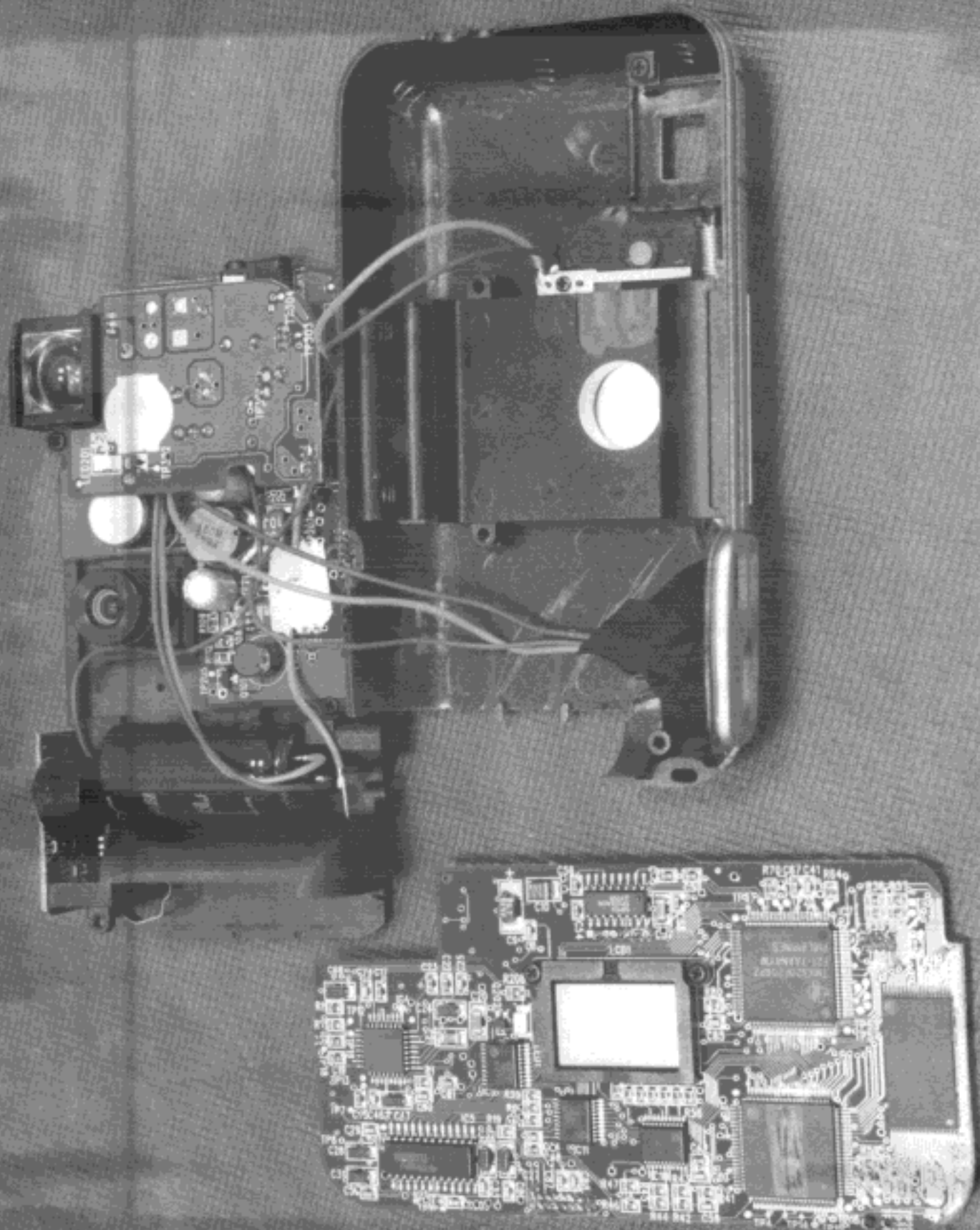
ECC ID : N3DLARGAND601A PHOTO 5. EUT INSIDE VIEW
