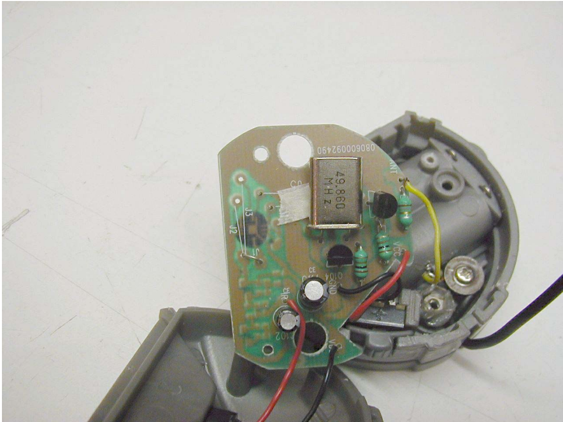
COMPONENT SIDE
