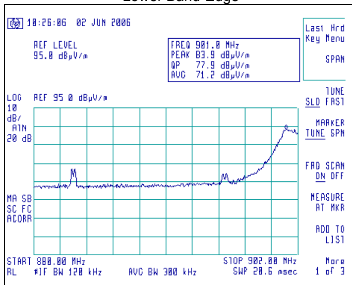
Lower Band-Edge
