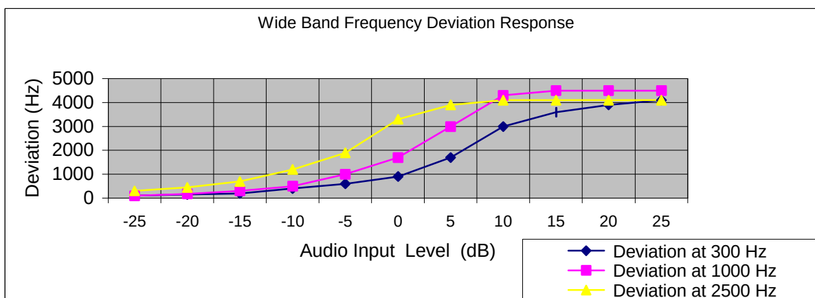
Figure 5: Deviation Characteristics.
