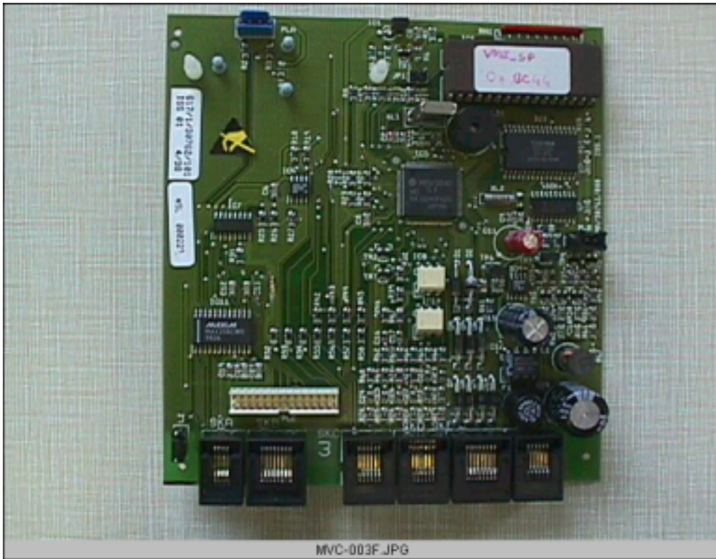
GPT Modem - Close Up of VIU PCB Component Side
