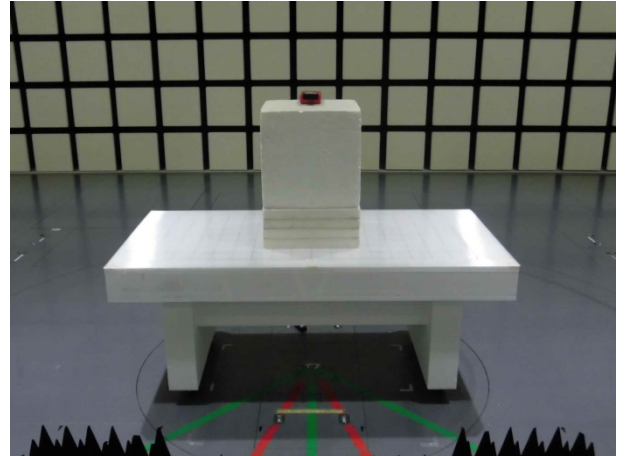
Above 1 GHz
