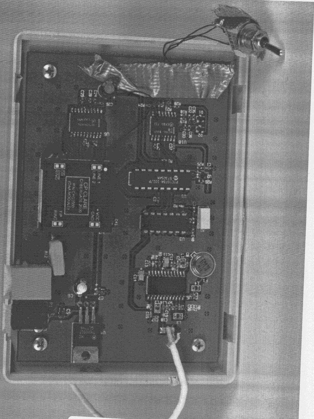
Lectron Technologies Project no.: 8R00115.2 Model: Lectron 20 Receiver FCC ID: N48202RECEIVER Component placement
