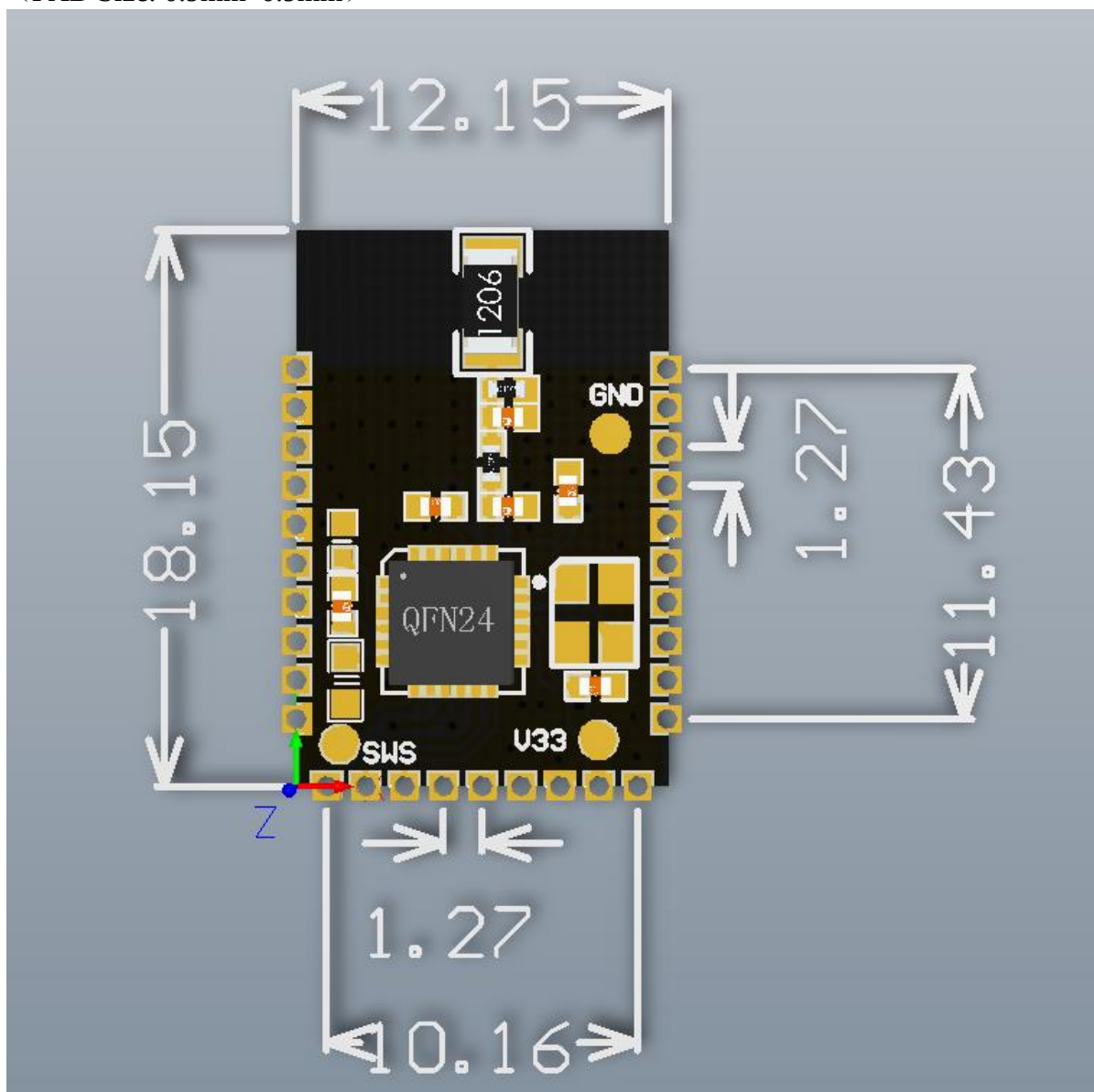
Fig.1 Packaging Drawing
