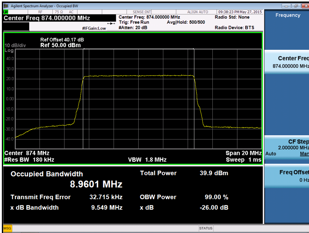
[Output DownlinkLow]
