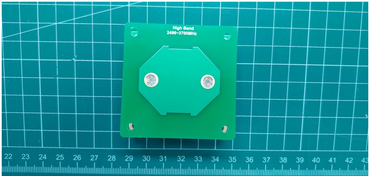
[ADXDLPR High Band Antenna (top)]
