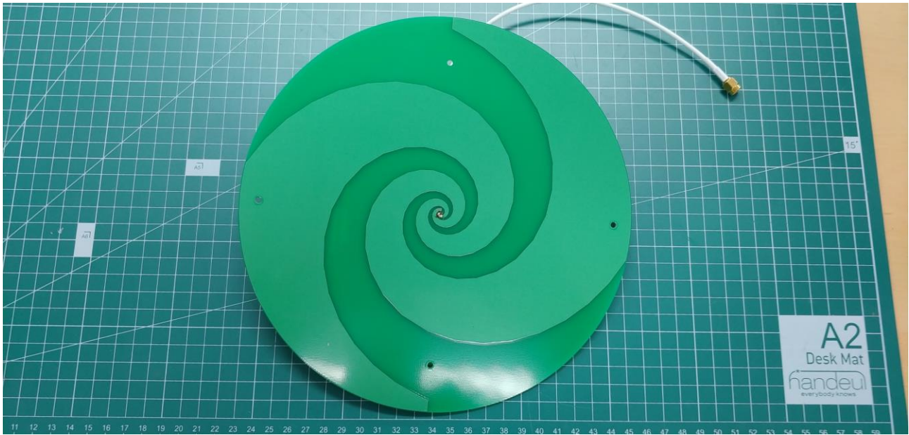
[ADXDLPR Low/middle Band Antenna (top)]
