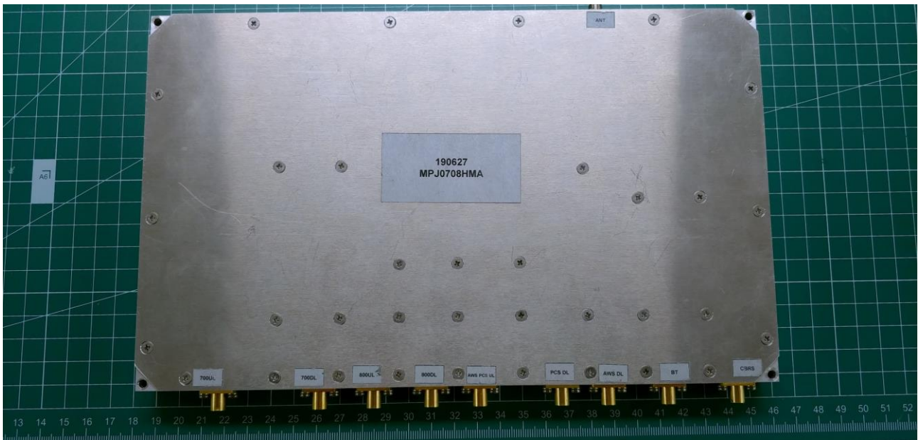
[ADXD-LPR Multiplexer (top)]
