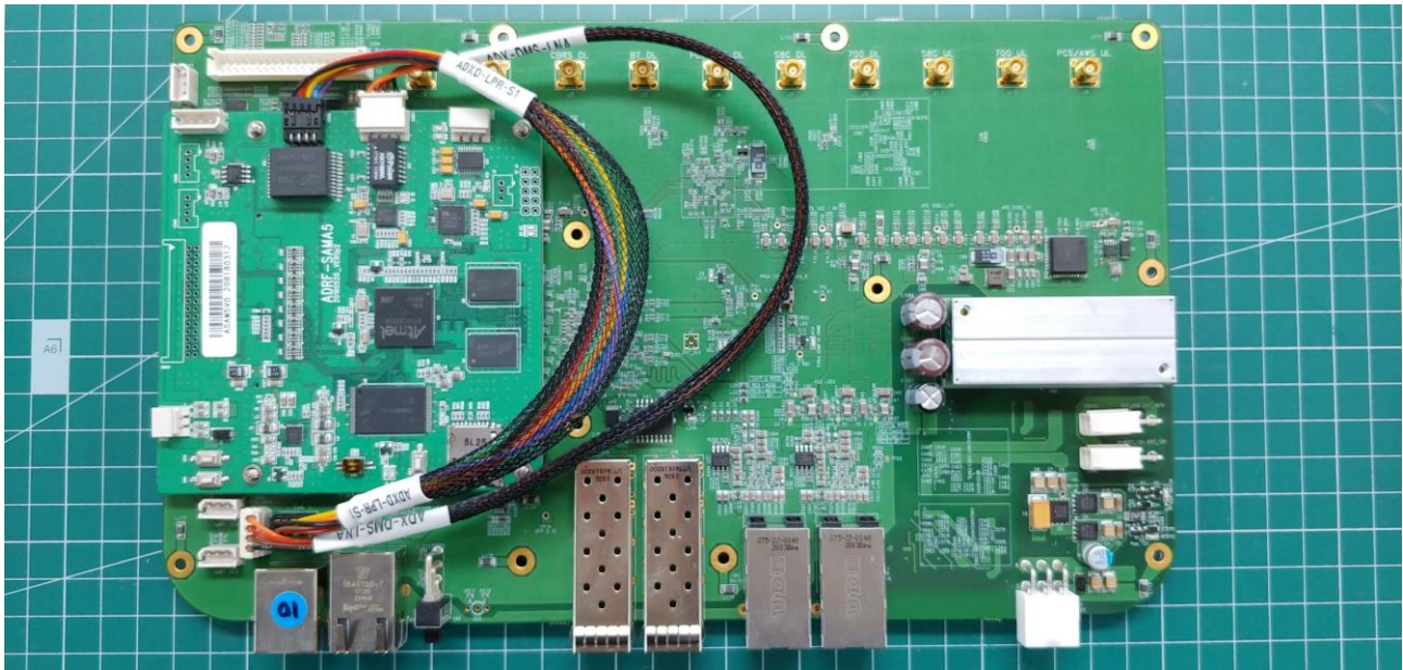
[ADXD-LPR Controller Board (top)]
