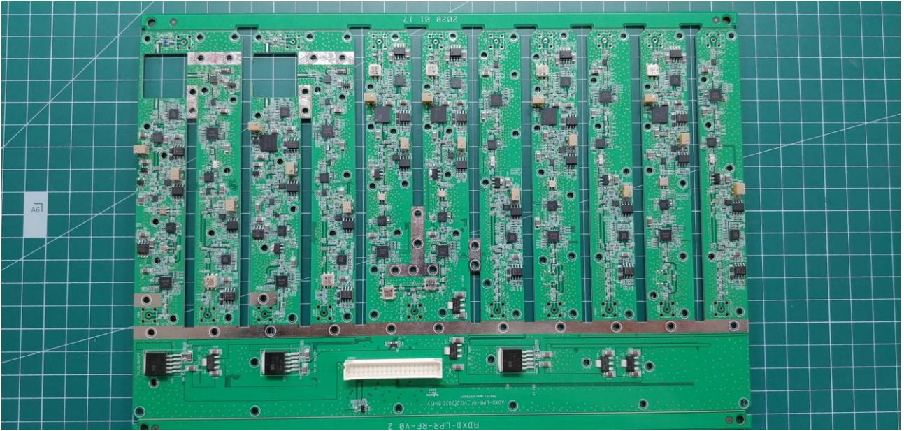
[ADXDLPR RF Board (top)]
