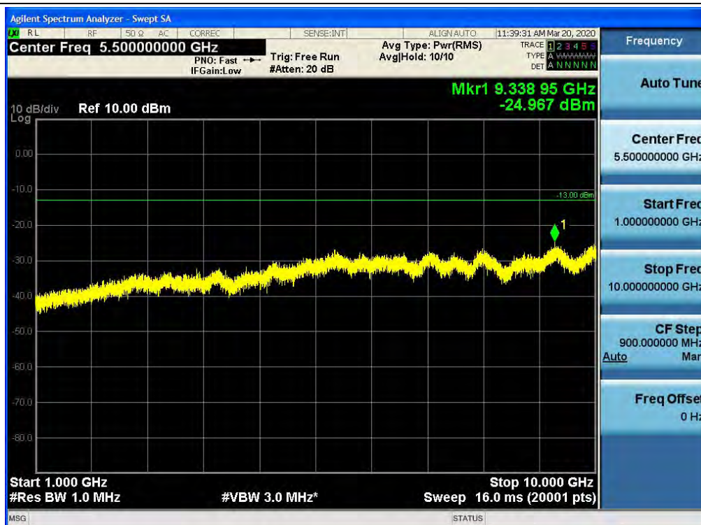
Spurious / Cellular / Downlink / LTE 20 MHz / Middle / 1 GHz ~ 10 GHz
