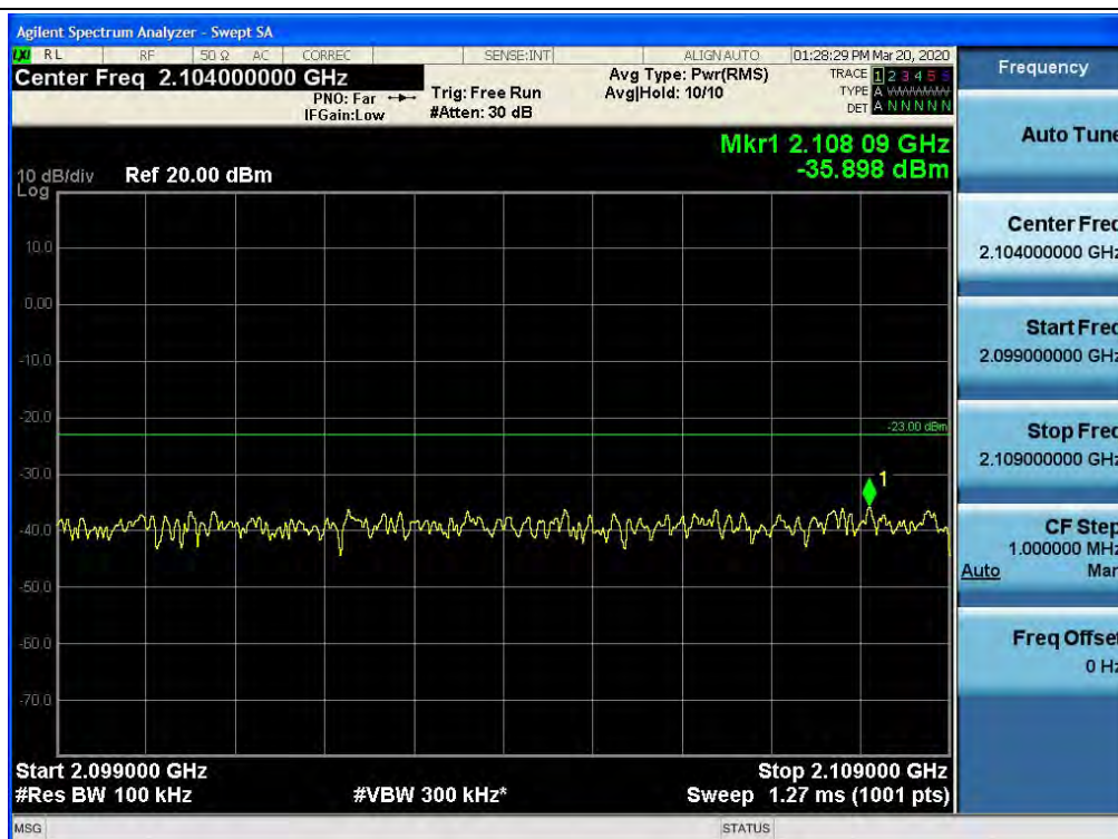
Spurious / AWS-1 / Downlink / LTE 20 MHz / Low / Low Edge-10 ~ Low Edge
