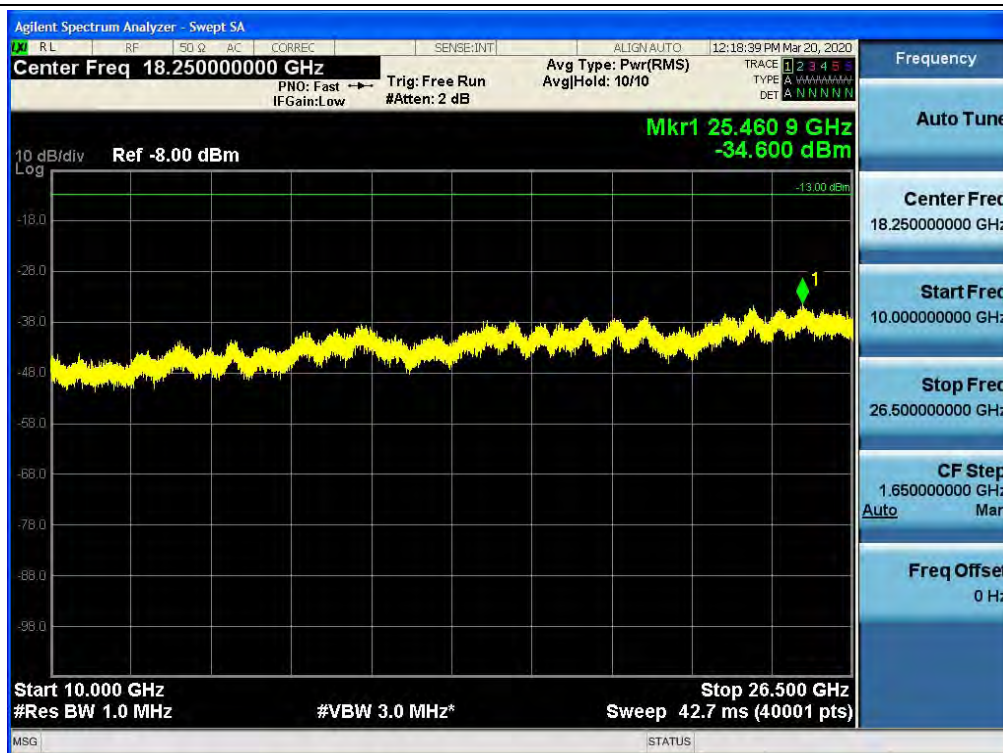
Spurious / Broadband PCS / Downlink / LTE 20 MHz / Low / 10 GHz ~ 26.5 GHz
