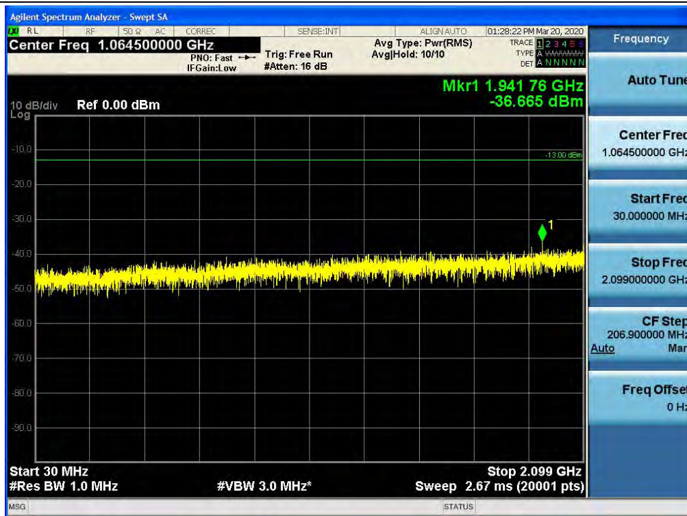
Spurious / AWS-1 / Downlink / LTE 20 MHz / Low / 30 MHz ~ Low Edge-10
