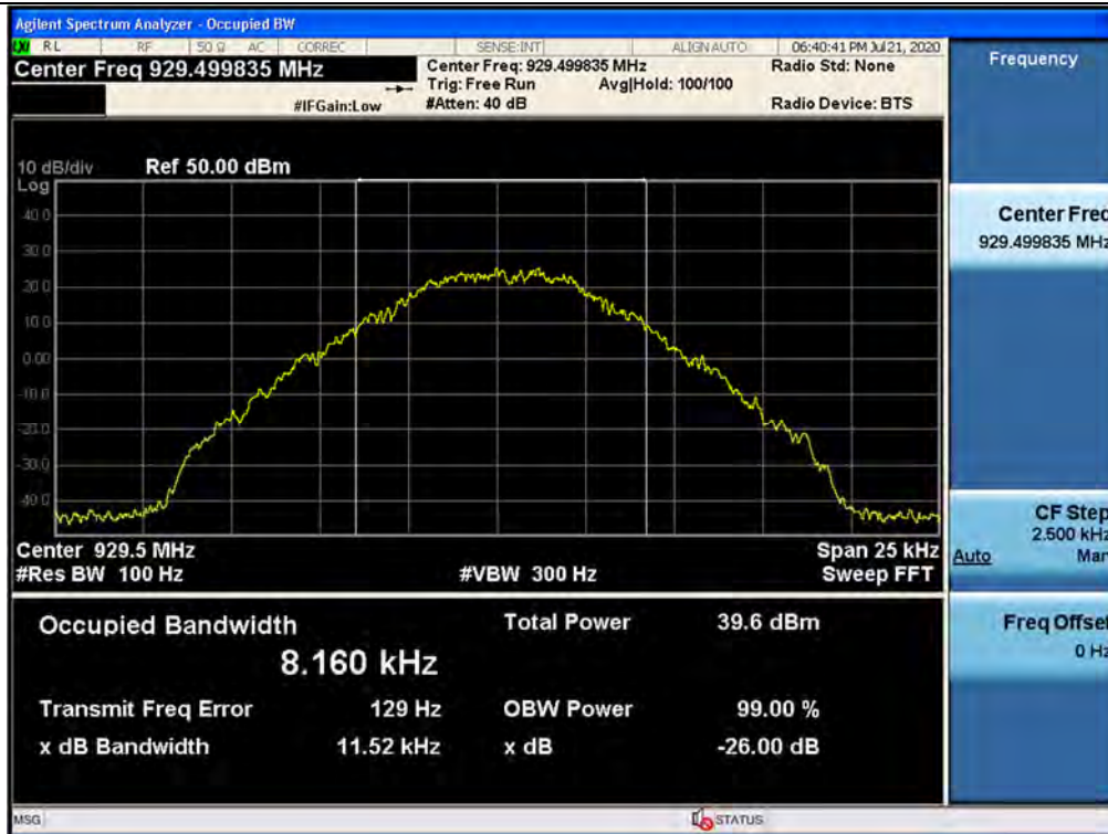
3 dB above the AGC threshold output / 929 ~ 930 MHz / Downlink / P25 Phase 1
