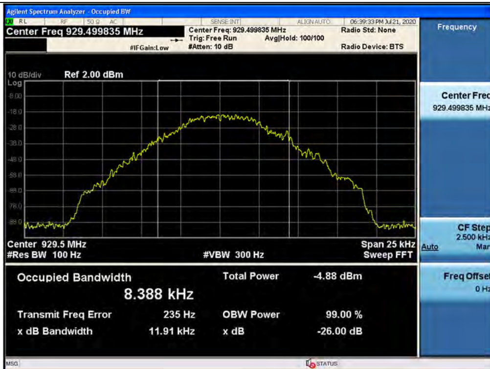
3 dB above the AGC threshold Input / 929 ~ 930 MHz / Downlink / P25 Phase 1
