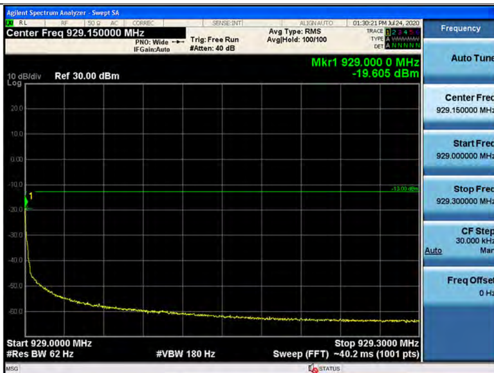
Out-of-band (single test signals) / 928 ~ 929 MHz / Downlink / P25 Phase 2 / Upper
