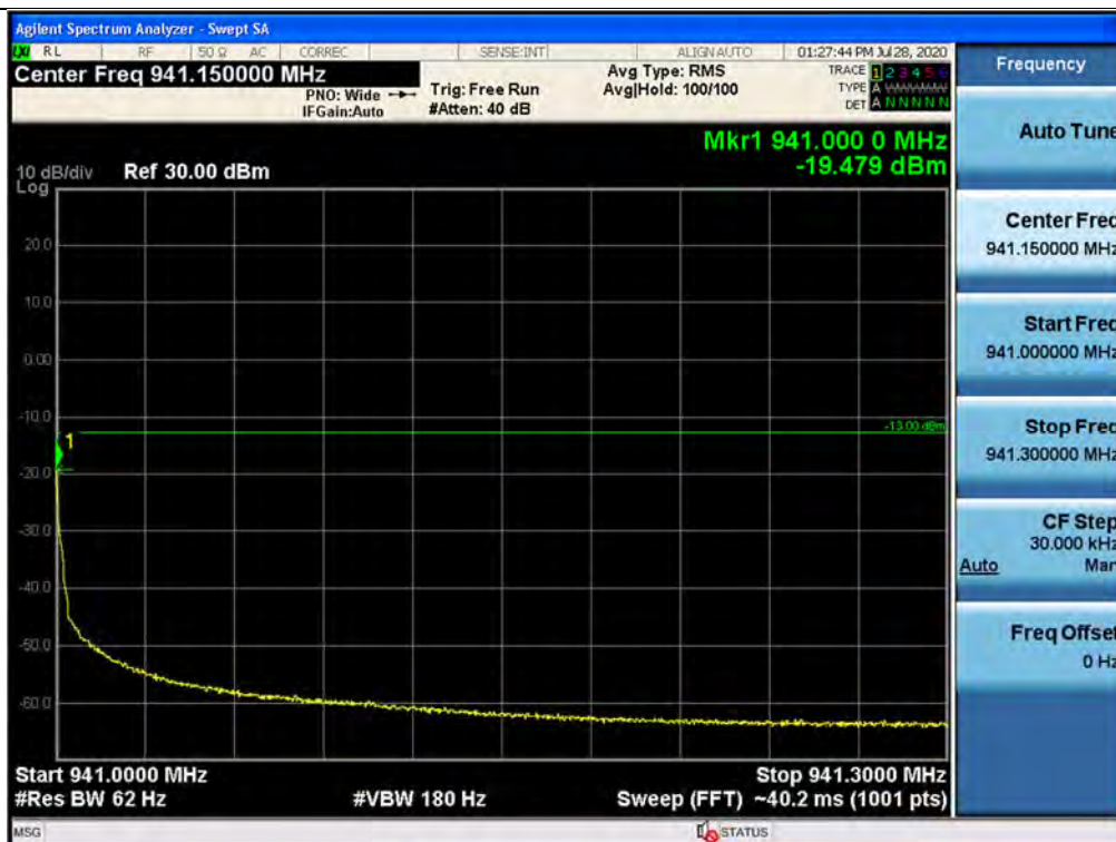
Out-of-band (single test signals) / 940 ~ 941 MHz / Downlink / P25 Phase 2 / Upper
