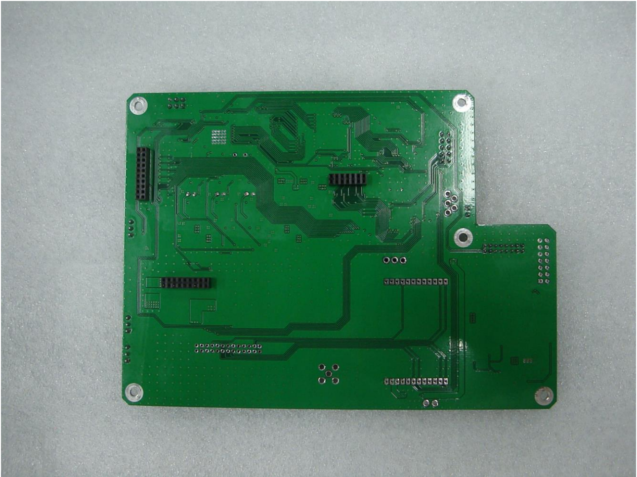
[CTRL B'd-BOT]
