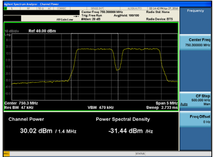
[700 MHz_Upper Downlink Mid]
