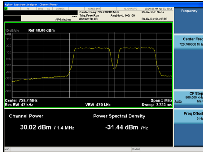
[700 MHz_Lower Downlink High]
