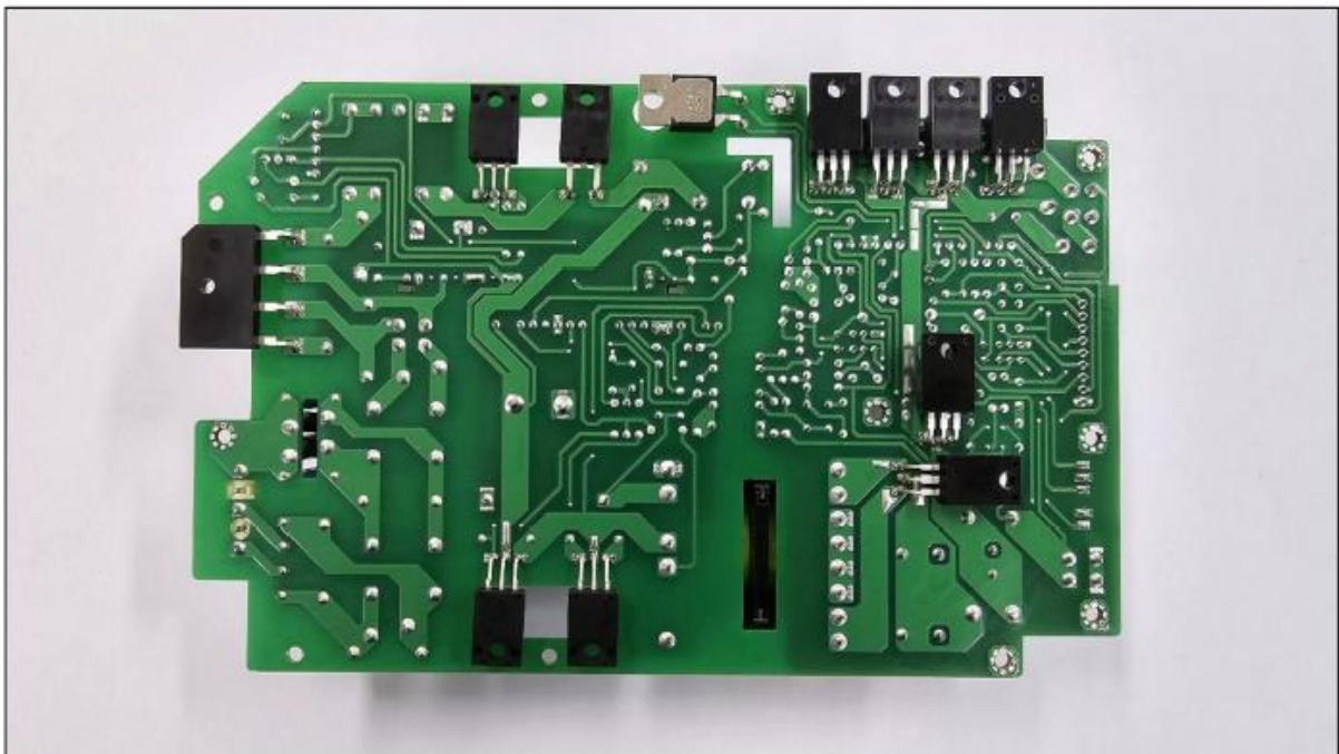
MAIN PCB Bottom
