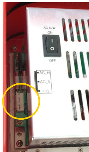
Figure 3-4 AC Terminal of the PSU
