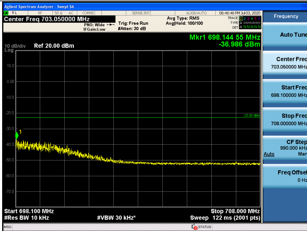
Spurious / 600 MHz Service / Uplink / 5G NR 20 MHz / High / High Edge ~ High Edge + 10 MHz
