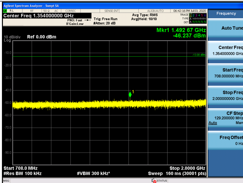
Spurious / 600 MHz Service / Uplink / 5G NR 20 MHz / Low / High Edge + 10 MHz ~ 2 GHz
