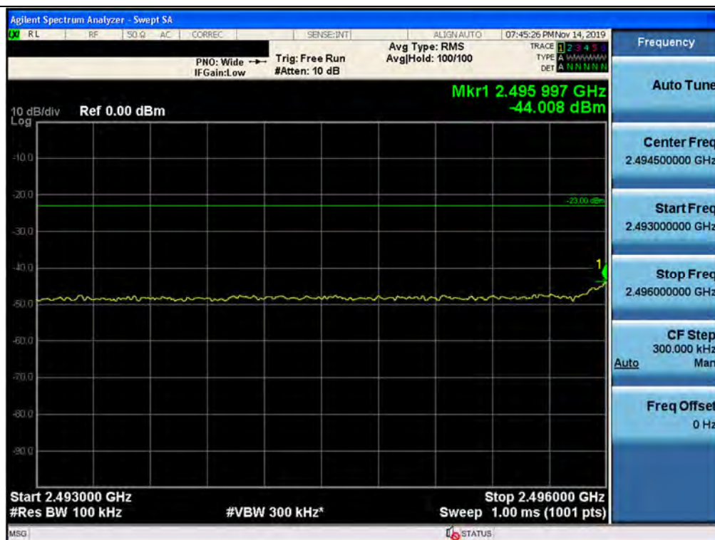
Out-of-band (single test signals) / BRS/EBS / Downlink / 5G NR 100M / Lower
