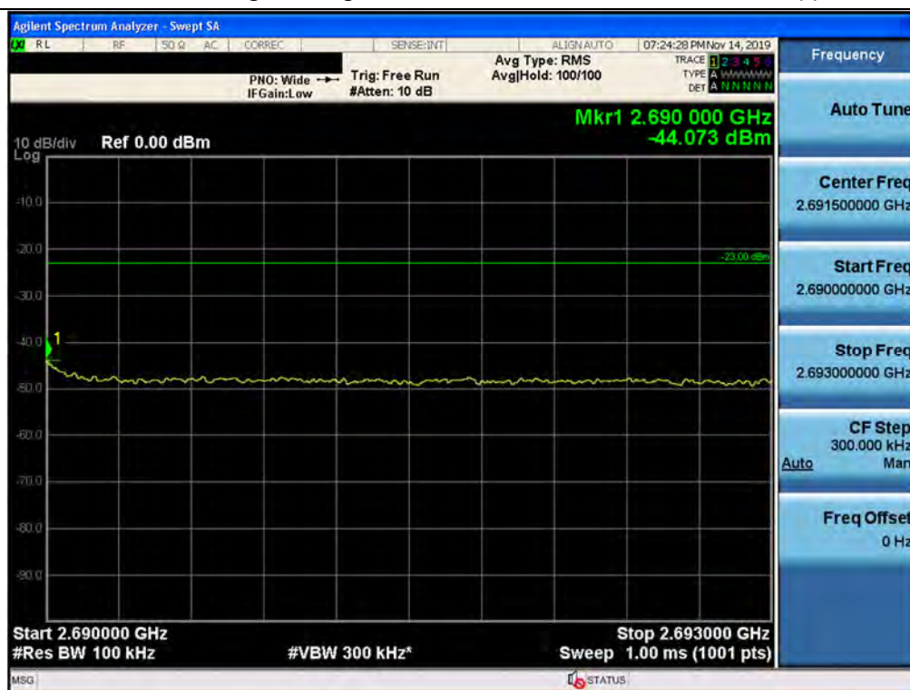
Out-of-band (single test signals) / BRS/EBS / Downlink / 5G NR 100M / Upper
