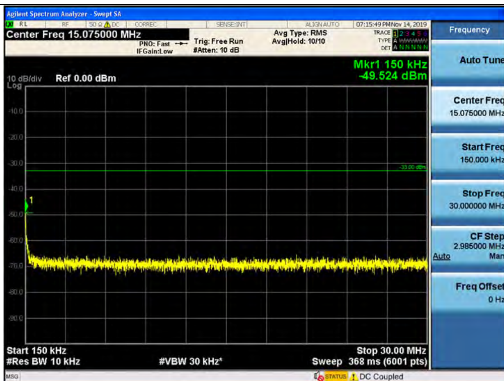
Spurious / BRS/EBS / Downlink / 5G NR 100M / Middle / 150 kHz ~ 30 MHz
