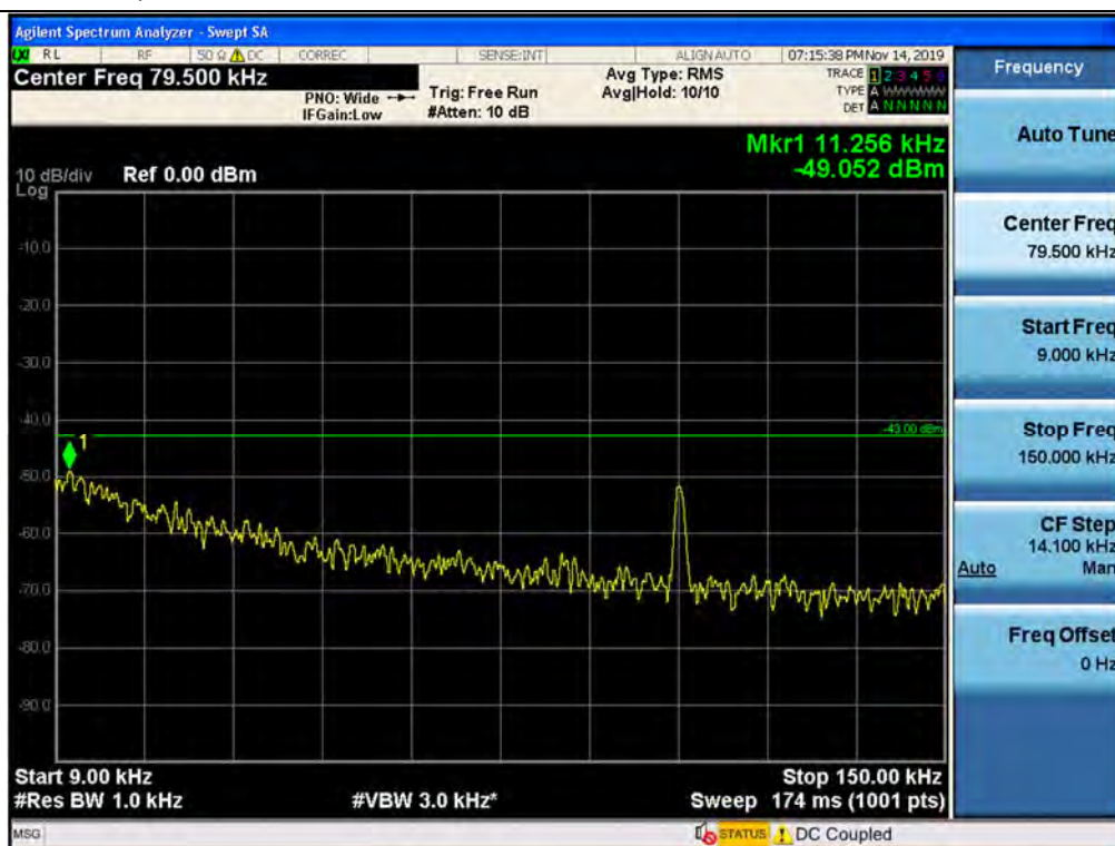
Spurious / BRS/EBS / 5G NR 100M / LTE 20 MHz / Middle / 9 kHz ~ 150 kHz
