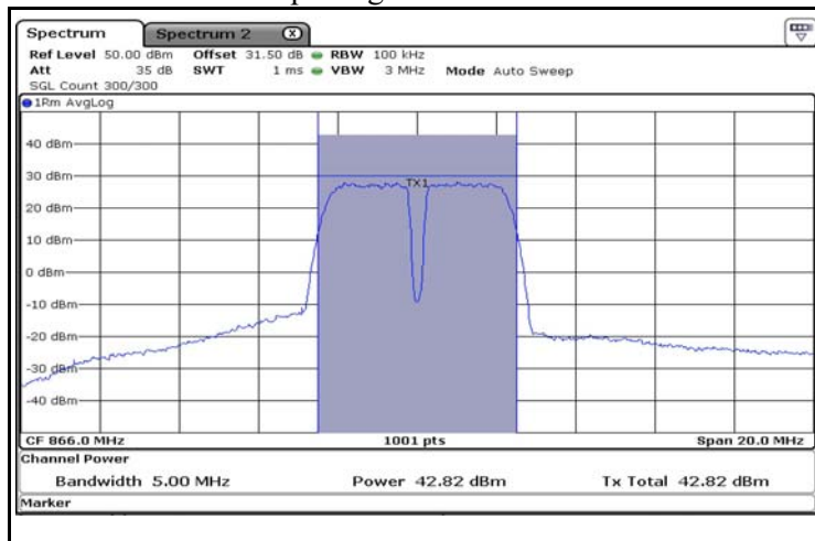
Output Signal of Downlink
