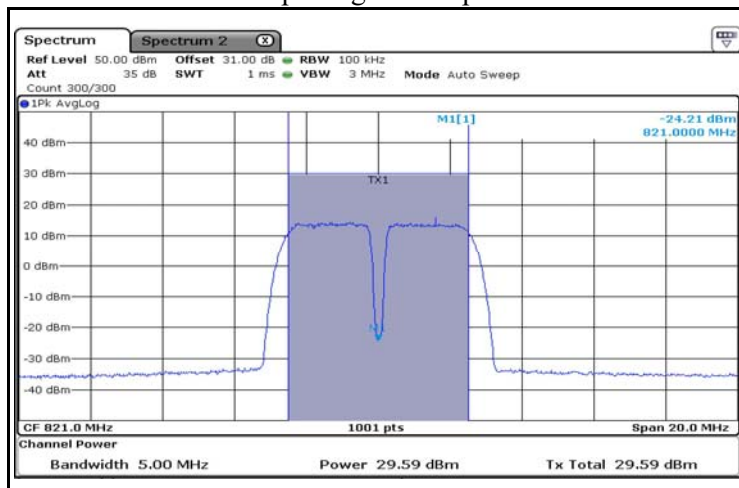
Output Signal of Uplink
