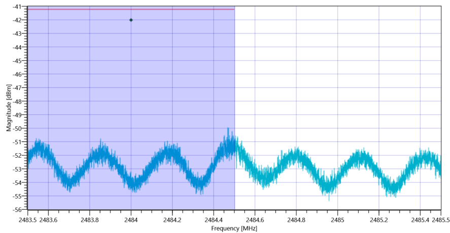
FCC Part 15.247 Restricted Band Edge Conducted Avg DC corrected DTS (eirp) ~ WLAN2G4 nHT40-mode
