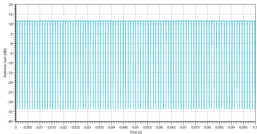
FCC Part 15.247 Restricted Band Edge Conducted Avg DC corrected DTS (eirr) ~ WLAN2G4 nHT40-mode 2452 MHz - DutyCycle
