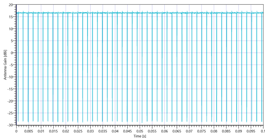
FCC Part 15.247 Restricted Band Edge Conducted Avg DC corrected DTS (eirr) ~ WLAN2G4 nHT20-mode 2412 MHz - DutyCycle
