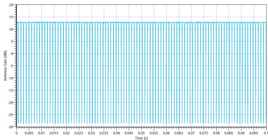
FCC Part 15.247 Restricted Band Edge Conducted Avg DC corrected DTS (eirr) ~ WLAN2G4 nHT40-mode 2422 MHz - DutyCycle
