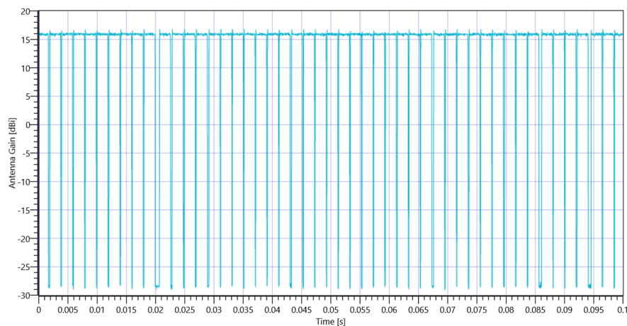
FCC Part 15.247 Restricted Band Edge Conducted Avg DC corrected DTS (eirr) ~ WLAN2G4 nHT20-mode 2462 MHz - DutyCycle
