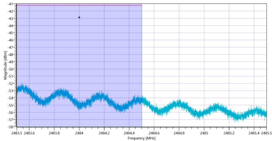
FCC Part 15.247 Restricted Band Edge Conducted Avg DC corrected DTS (eirp) ~ WLAN2G4 nHT20-mode
