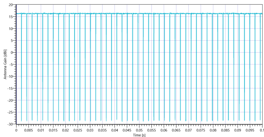
FCC Part 15.247 Restricted Band Edge Conducted Avg DC corrected DTS (eirr) ~ WLAN2G4 g-mode 2462 MHz - DutyCycle
