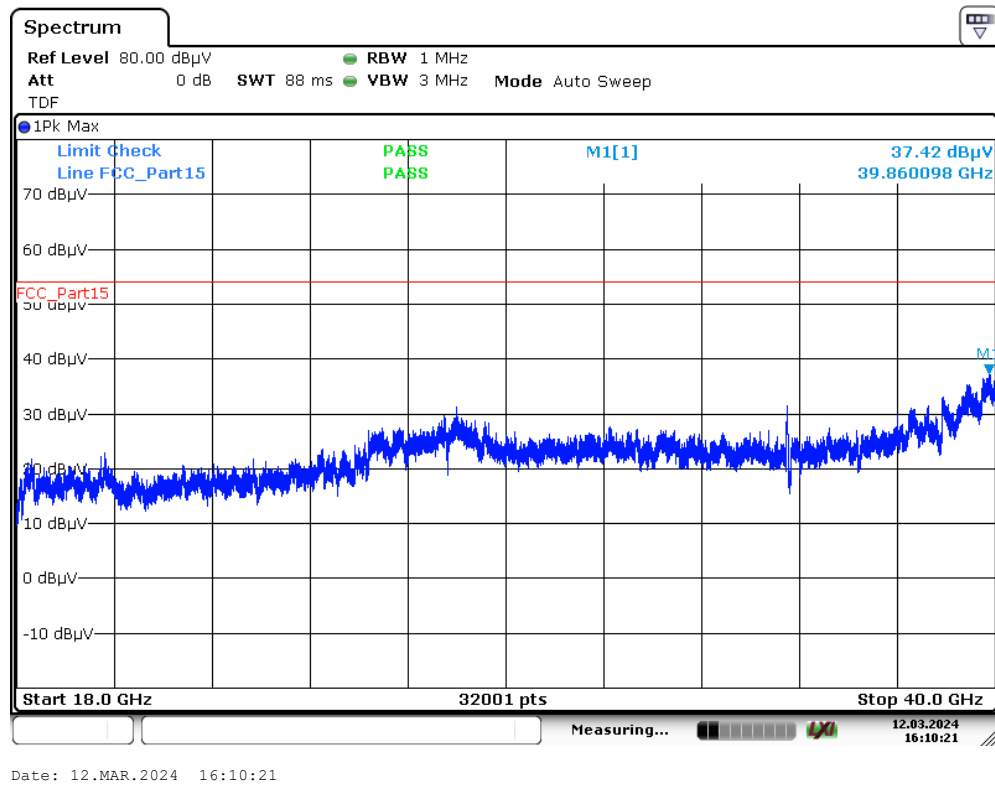
Plot 3: 18 GHz to 40 GHz; vertical & horizontal polarization; U-NII-3; valid for all channels and modes
