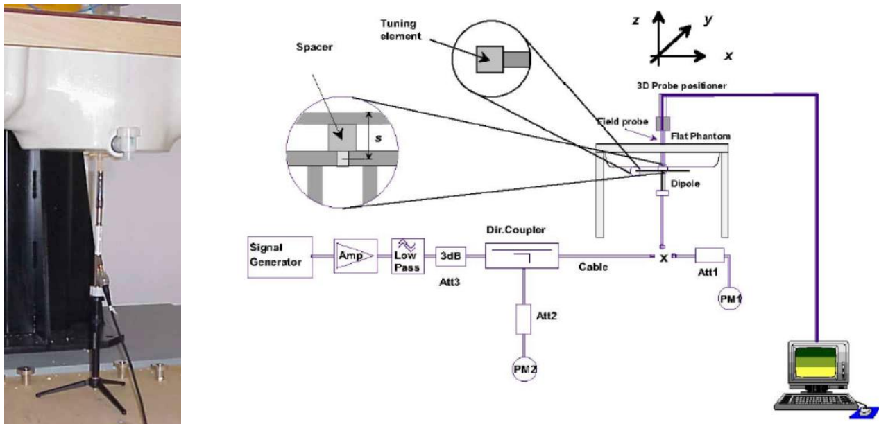
F-1. the microwave circuit arrangement used for SAR system check
