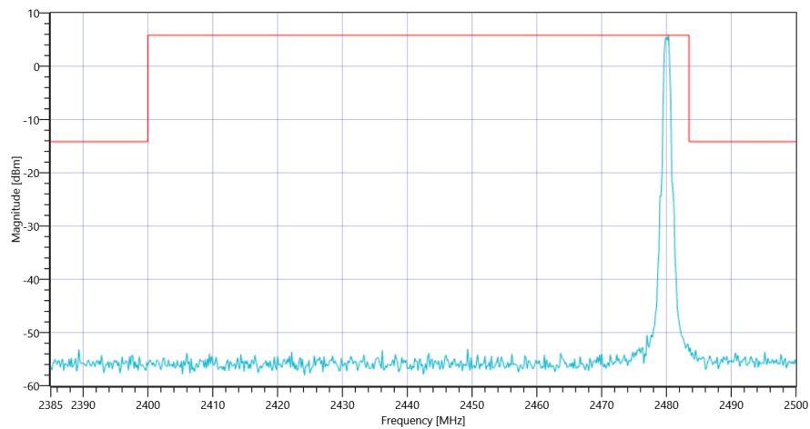
FCC Part 15.247 TX Spurious Conducted ~ BT LE 1 Msp 2480
