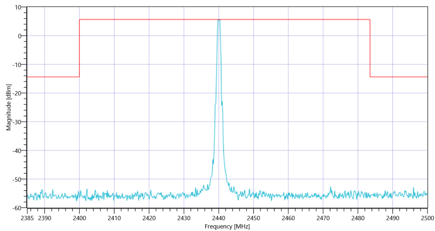
FCC Part 15.247 TX Spurious Conducted ~ BT LE 1 Msp 2440
