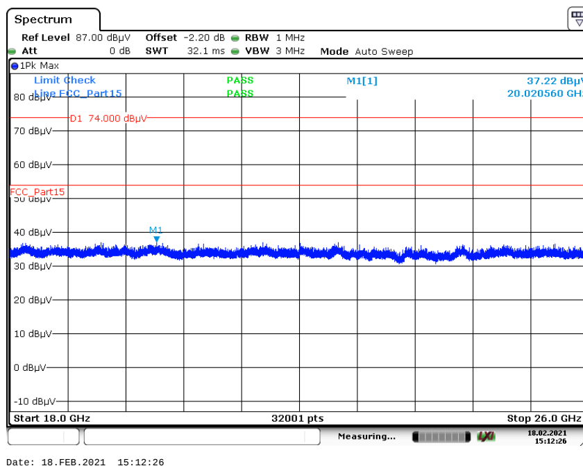
Plot 6: 18 GHz to 26 GHz, high channel, vertical & horizontal polarization, GFSK
