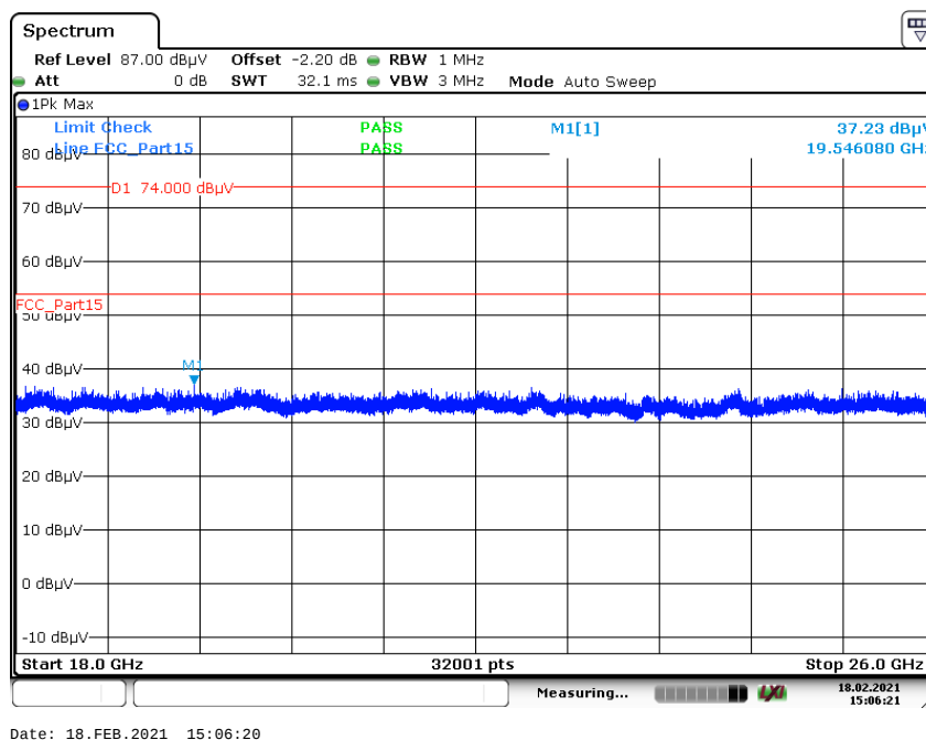
Plot 4: 18 GHz to 26 GHz, mid channel, vertical & horizontal polarization, GFSK
