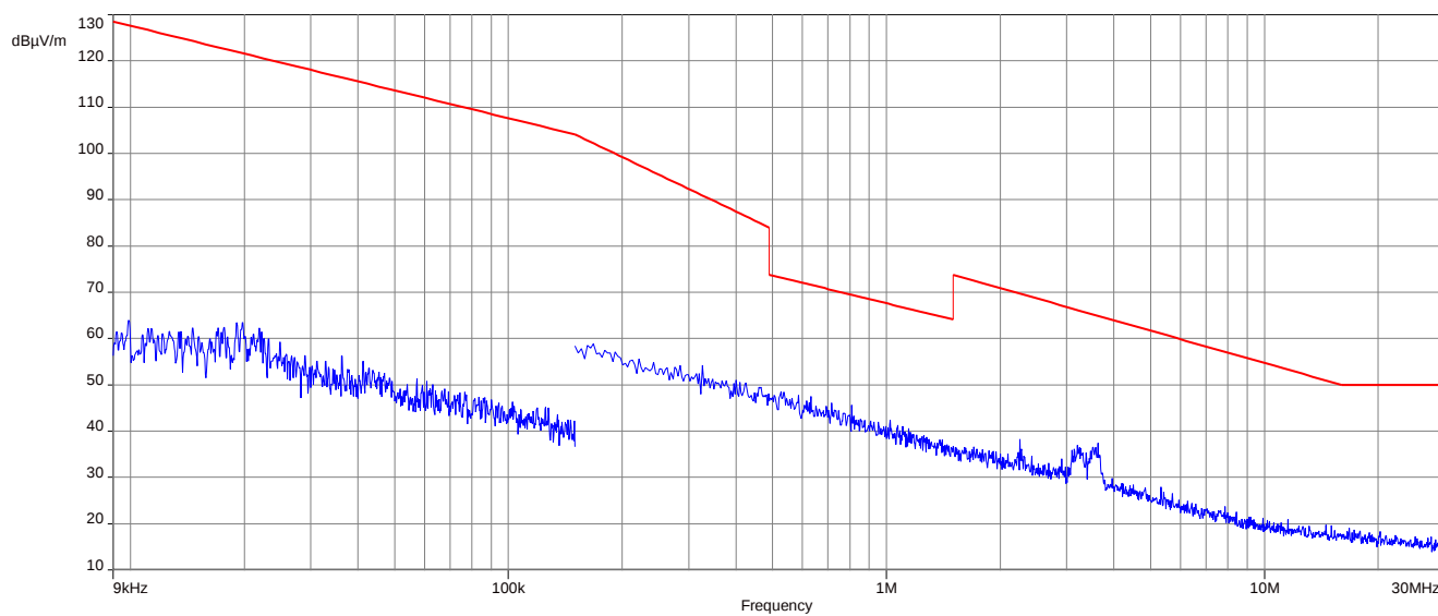
Plot 3: 9 kHz to 30 MHz, high channel, GFSK
