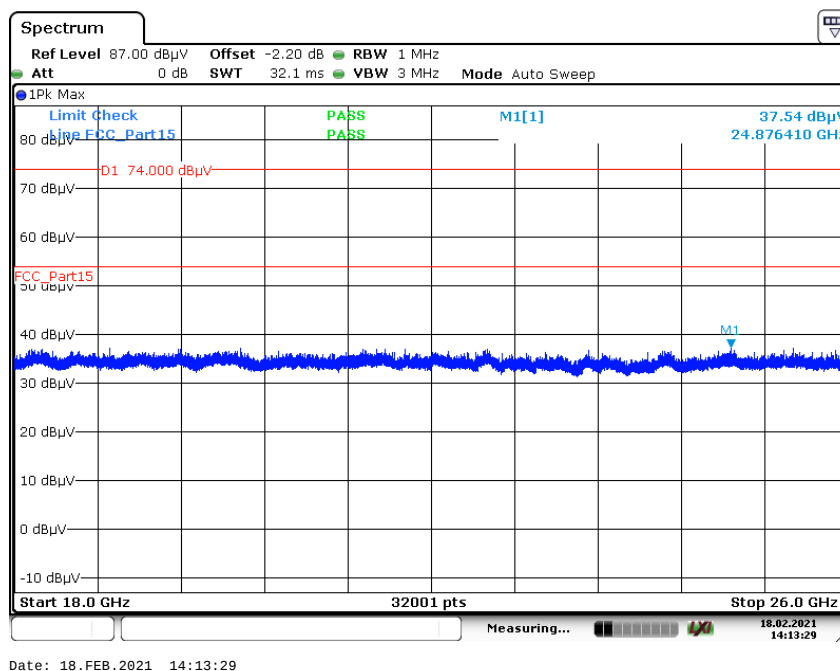
Plot 6: 18 GHz to 26 GHz, high channel, vertical & horizontal polarization, CW
